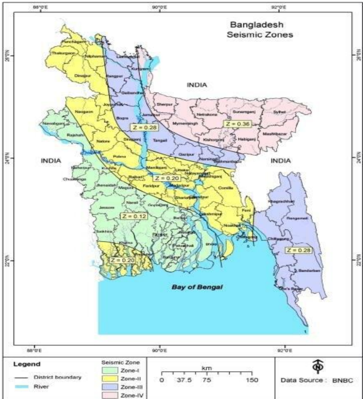
Figure 3: Seismic Zone Map of Bangladesh BNBC -2020
