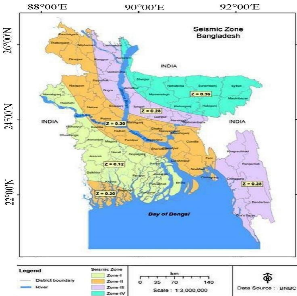
Figure 4: Seismic Zone Map of Bangladesh BNBC -202
