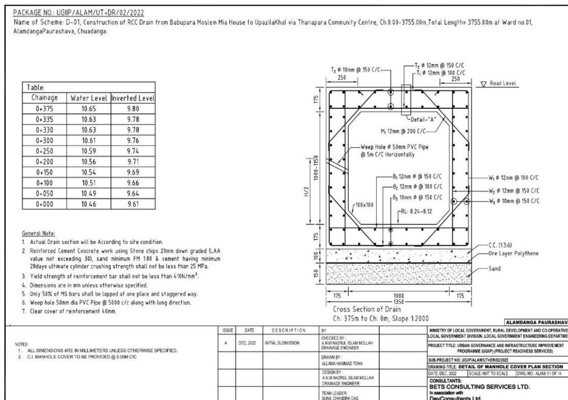
Figure 6: Cross-Section of Drain in Alamdanga Pourashava
