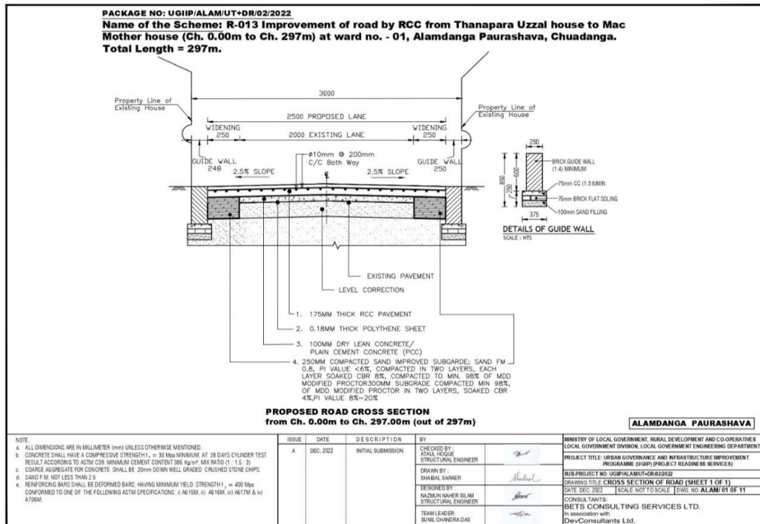
Figure 5: Cross-Section of Road in Alamdanga Pourashava
