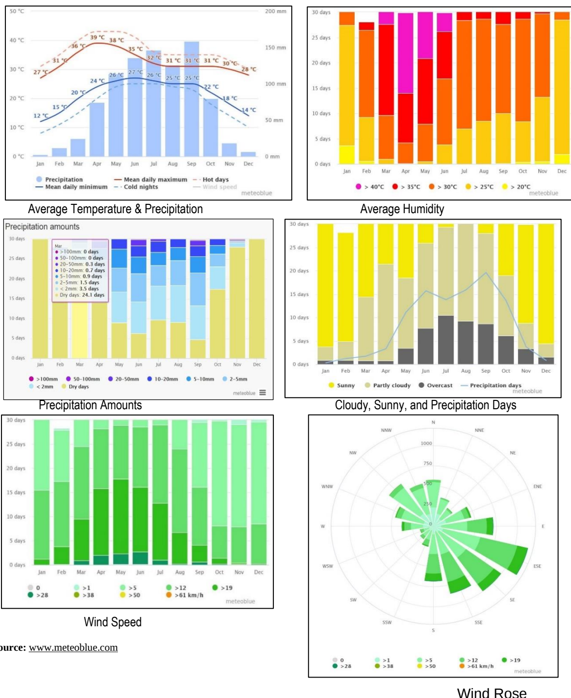
Figure 7: Historical Climatic Record at Alamdanga Region
