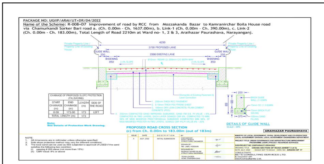
Figure III-3: Cross Section of Road in Araihaazar Pourashava
