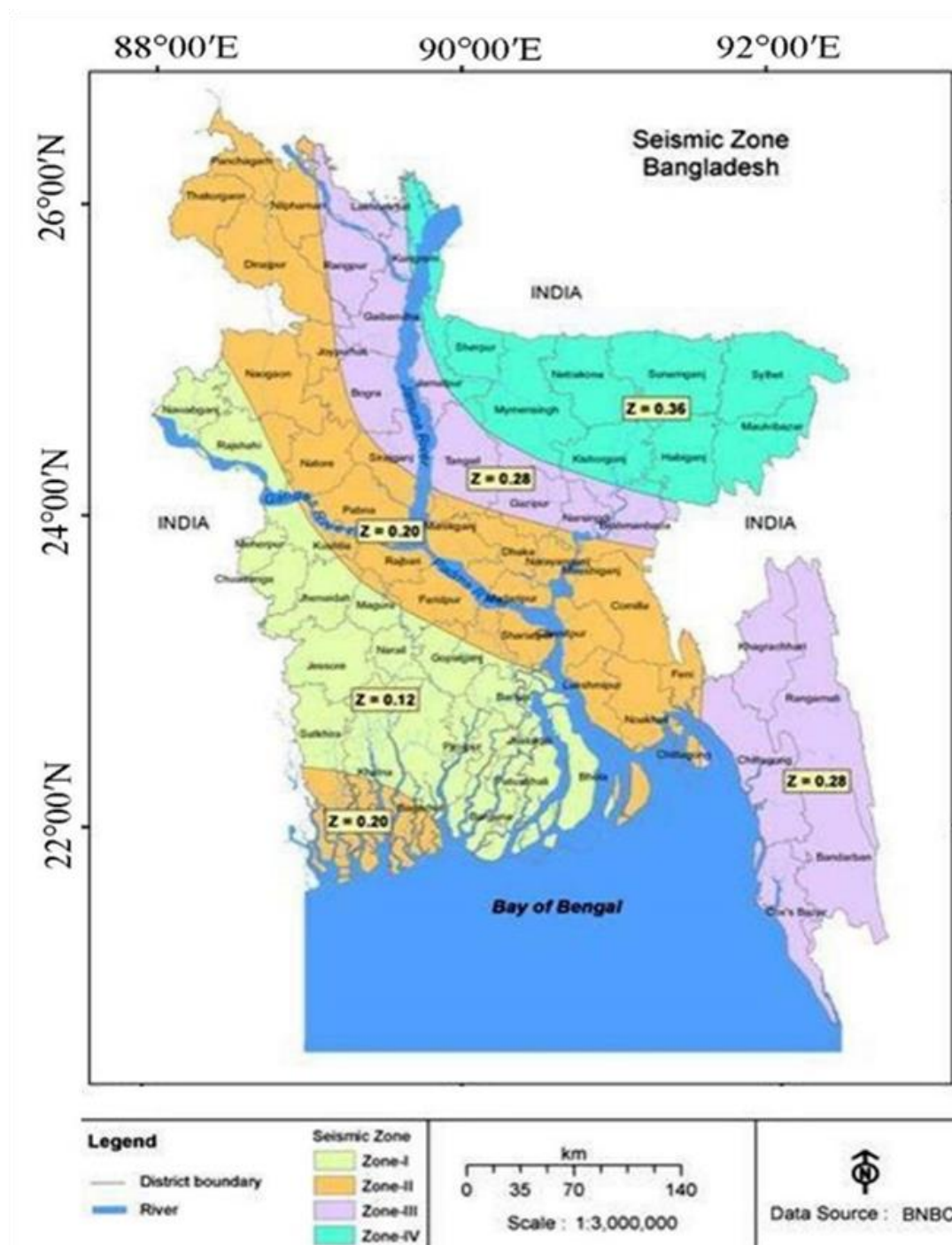
Figure IV-5: Seismic Zones of Bangladesh (4 Zones) [Source: BNBC]
