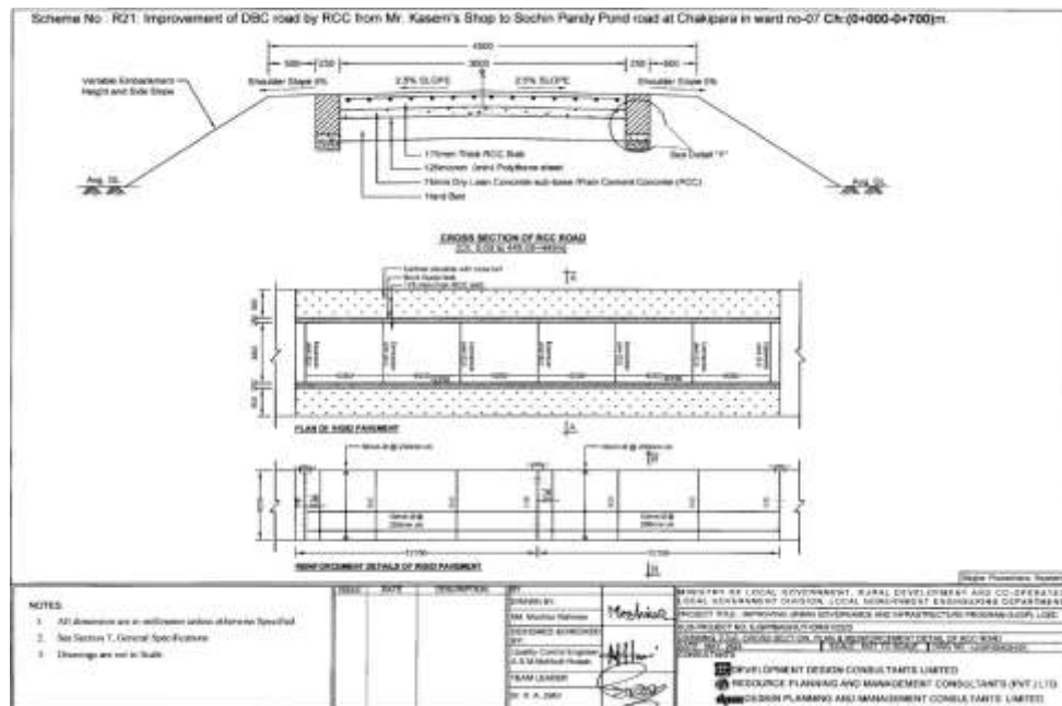
Figure 3: Cross-Section of Road in Pourashava
