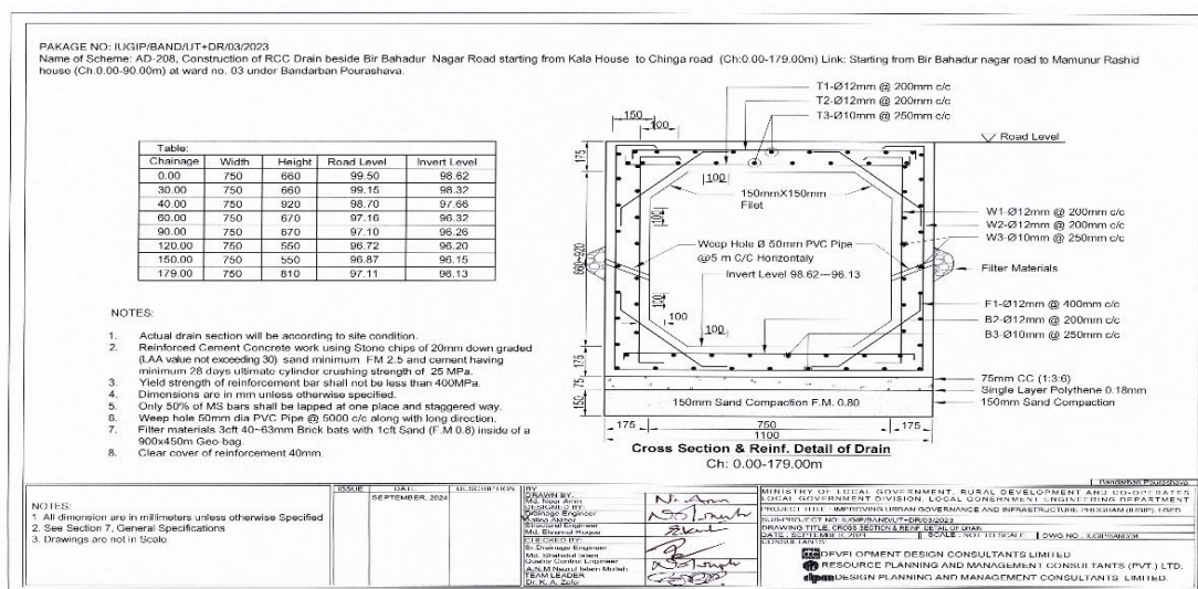
Figure III-4: Cross Section of Drain in Bandarban Pourashava
