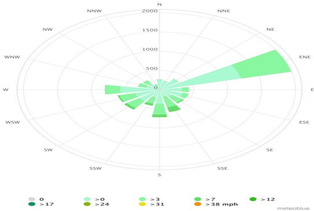
Figure IV-4: Wind Rose*
