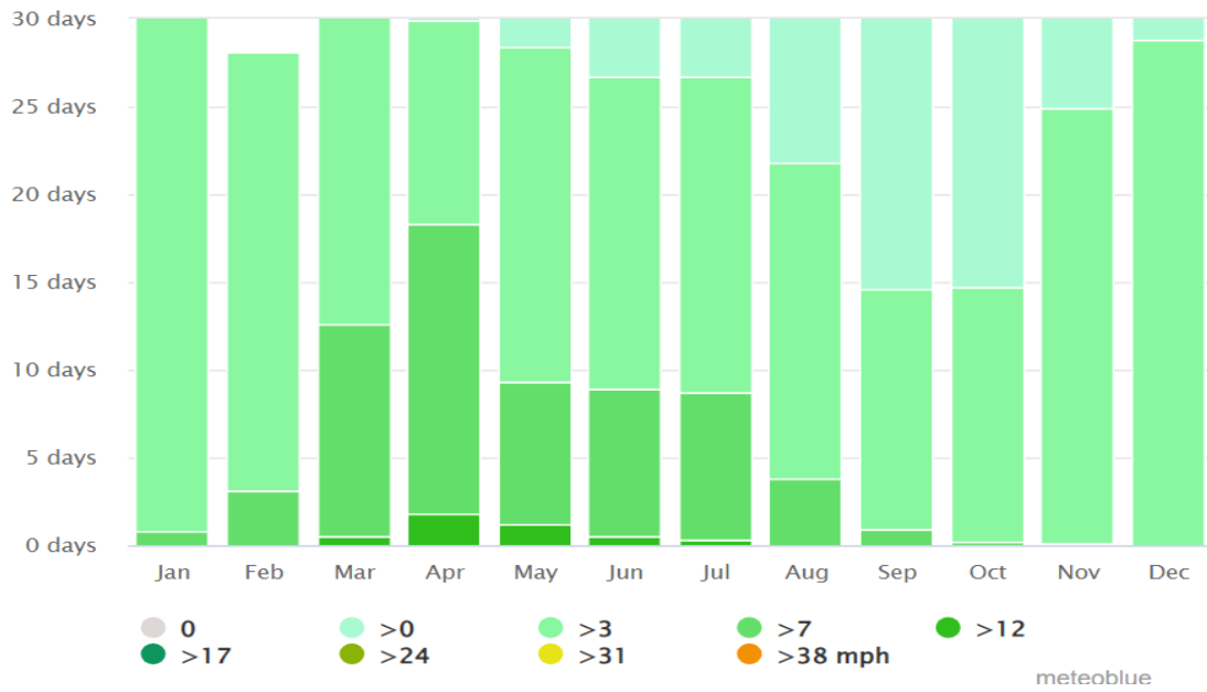
Figure IV-3: Wind Speed*
