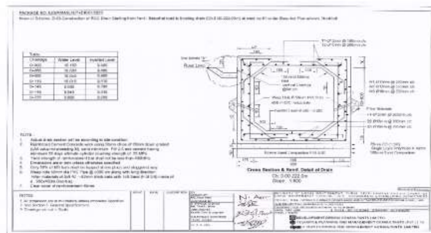
Figure III-4: Cross Section of Drain in Basurhat Pourashava
