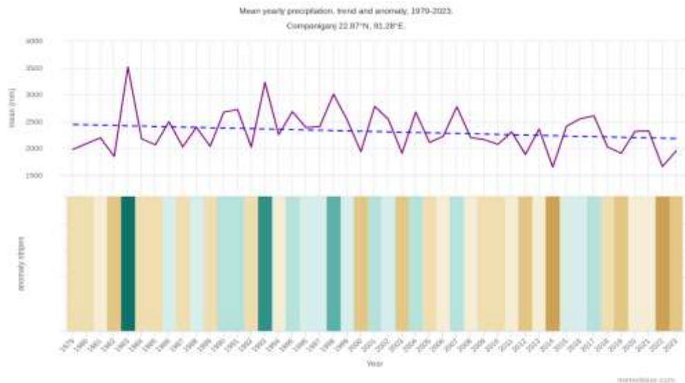
Figure IV-2: Yearly Precipitation Change*
