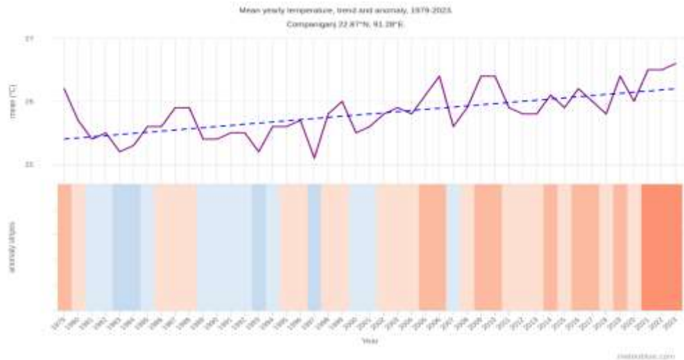
Figure IV-1: Yearly Temperature Change*
