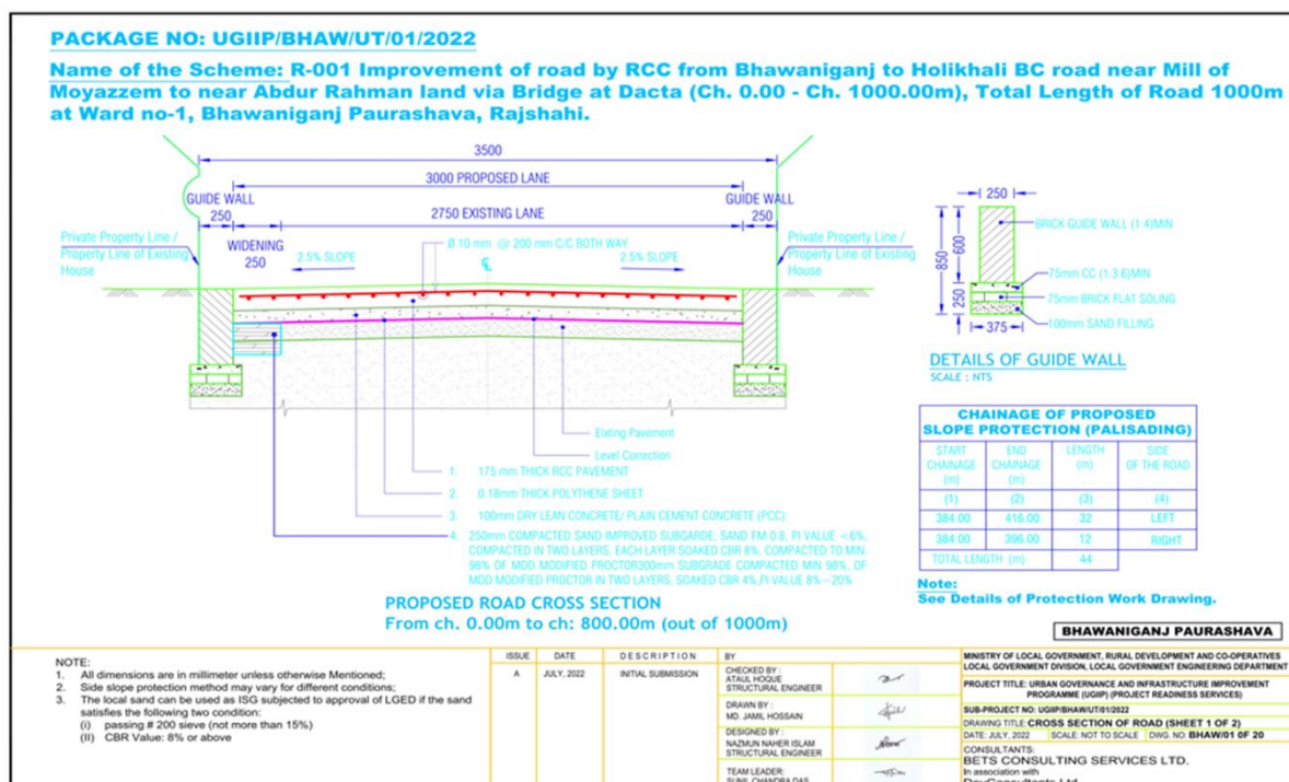
Figure 3: Cross-Section of Road Bhawaniganj Paurashava
