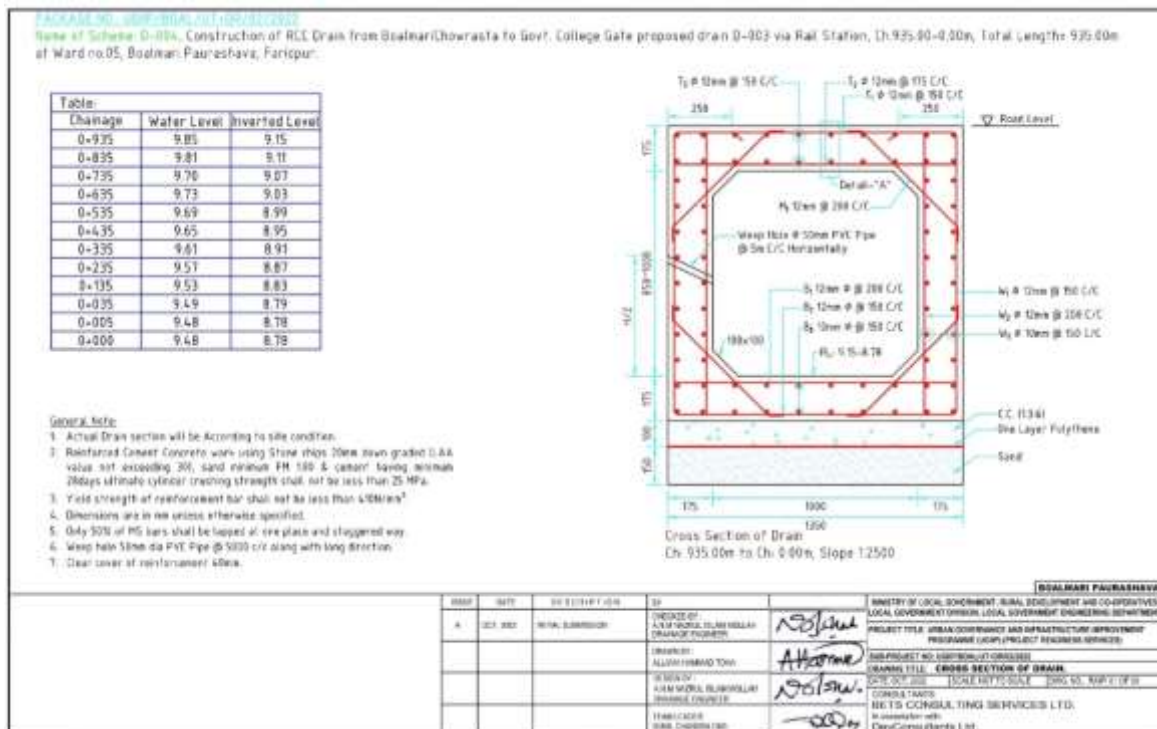
Figure 7: Cross-Section of Drain in Pourashava
