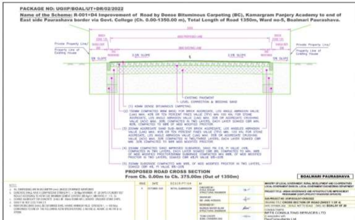
Figure 6: Cross-Section of Road in Pourashava
