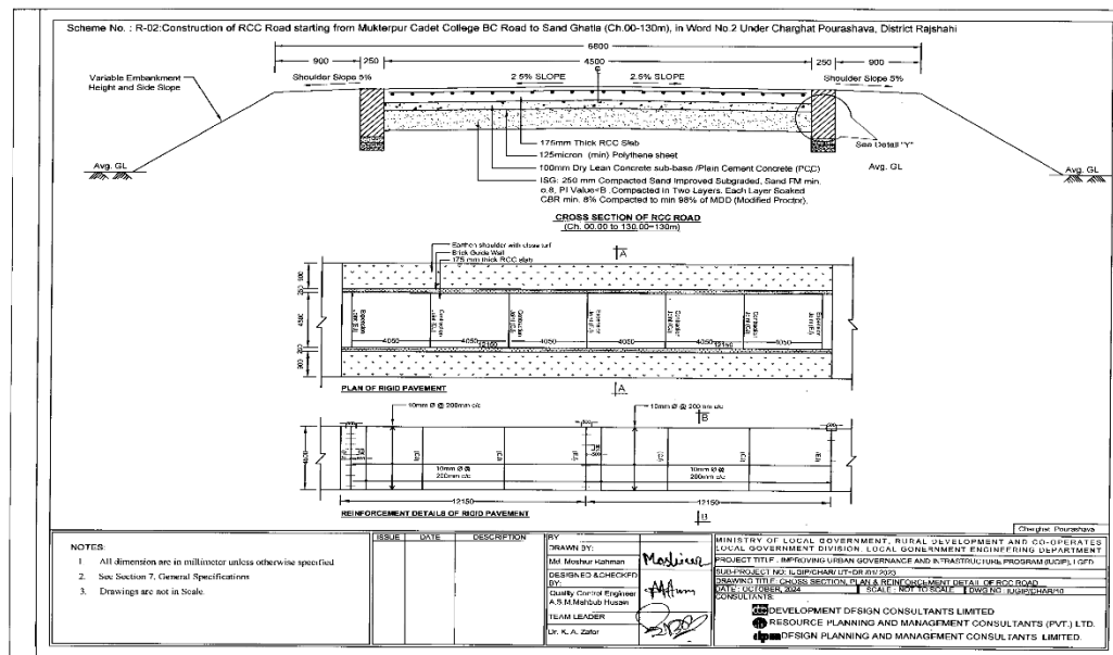
Figure 3: Cross-Section of Road in Pourashava
