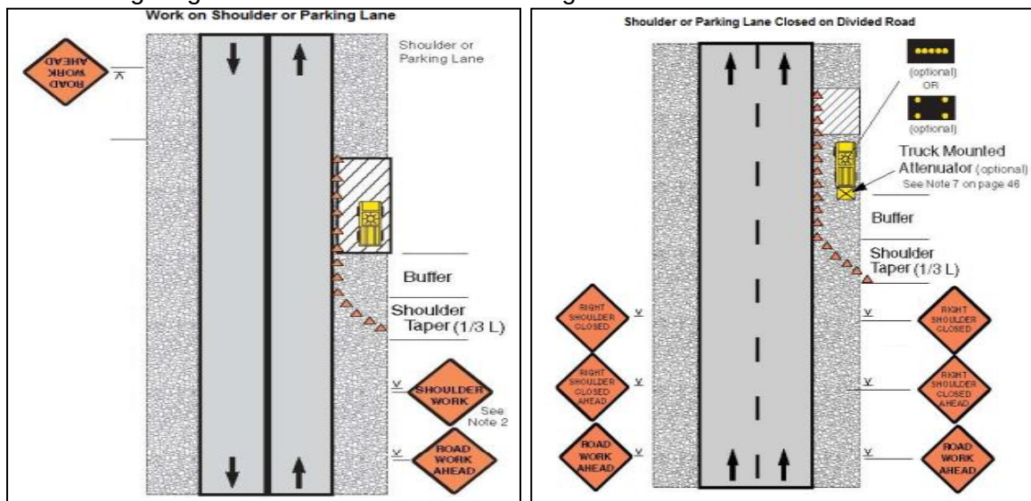
Figure A2 & A3: Work on shoulder or parking lane and shoulder or parking lane closed on divided road
