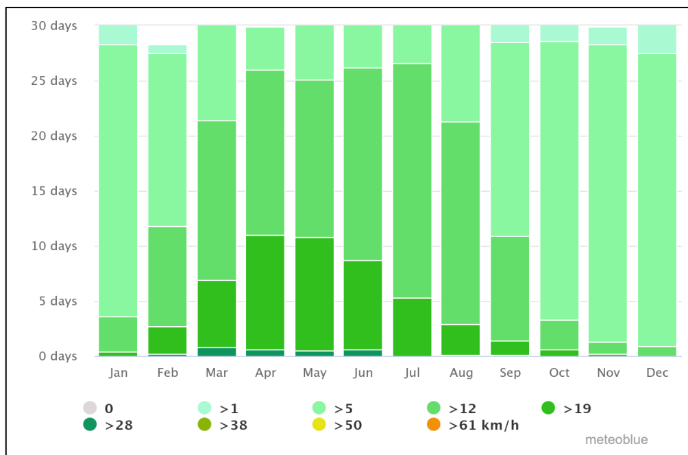
Figure IV-3: Wind Speed*
