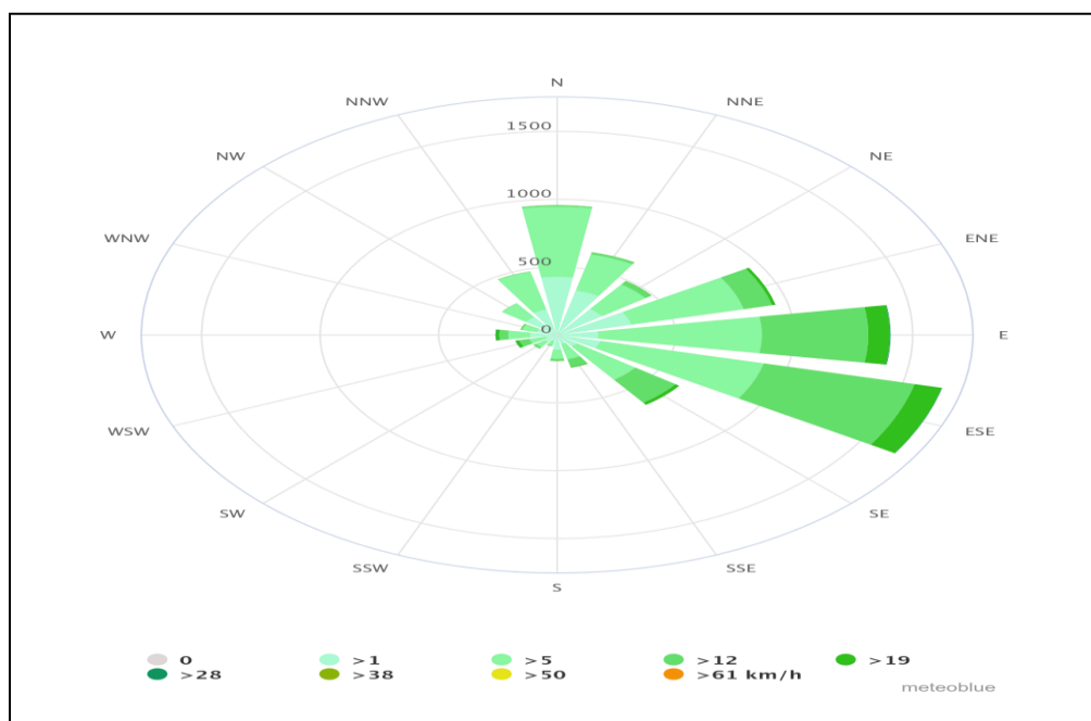
Figure IV-4: Wind Rose*
