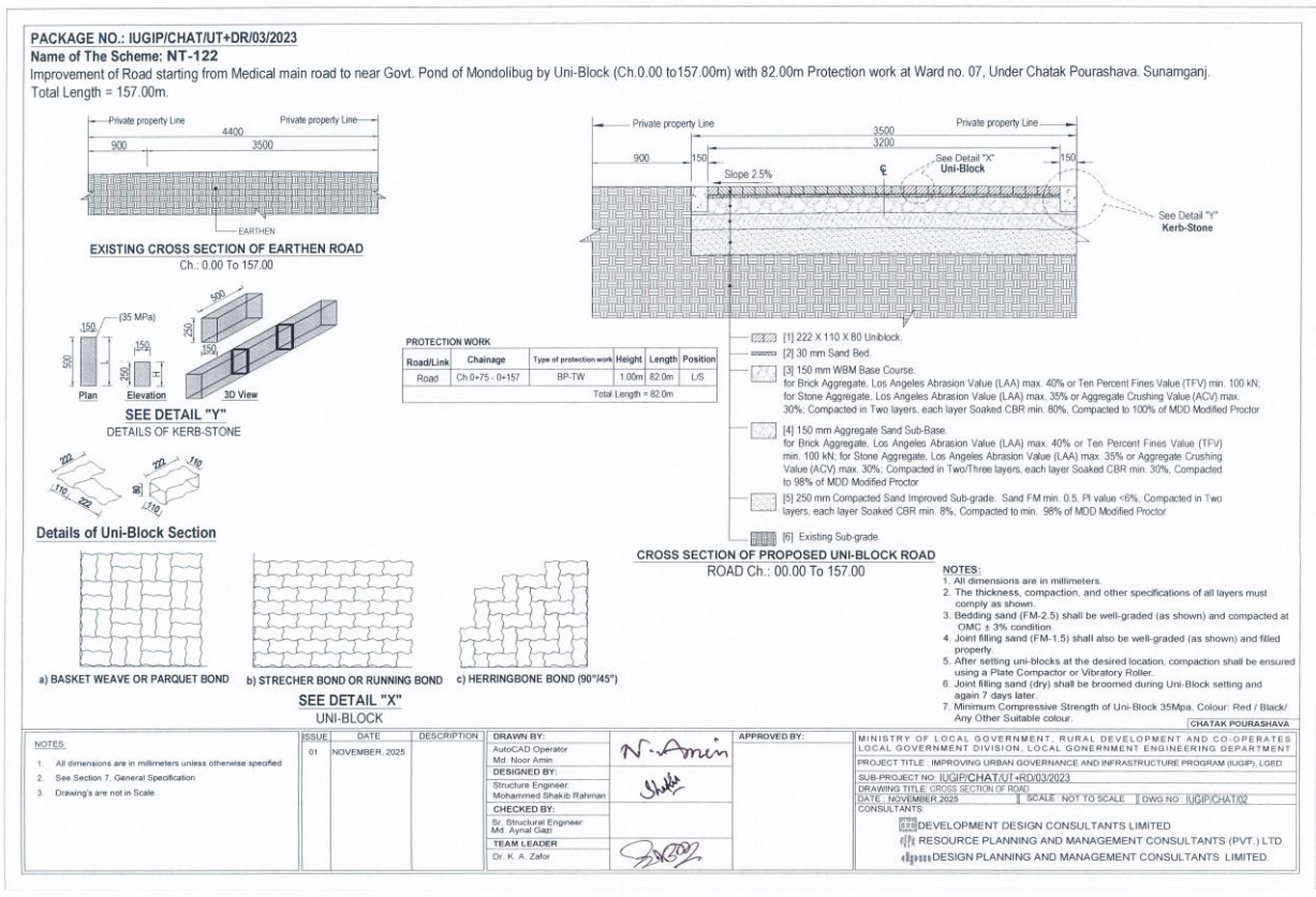
Figure III-3: Cross Section of Road in Chhatak Pourashava
