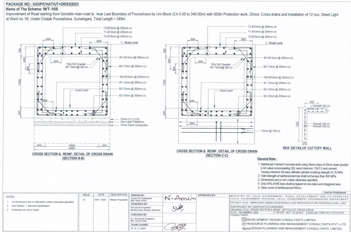
Figure III-4: Cross Section of Drain in Chhatak Pourashava
