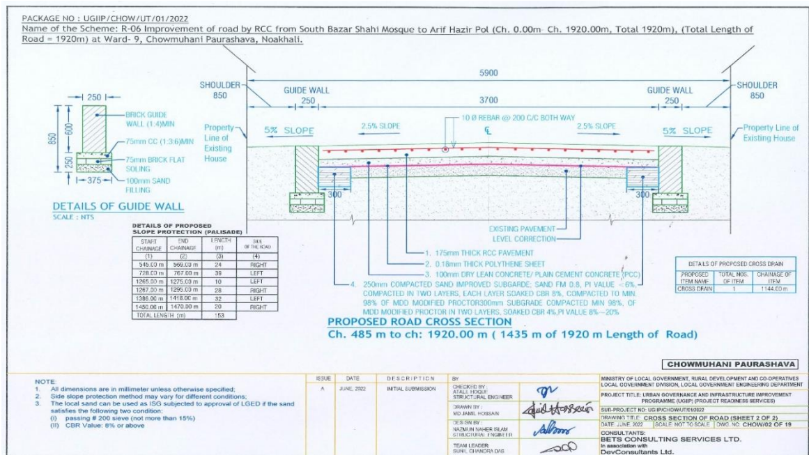
Figure 3: Cross-Section of Road
