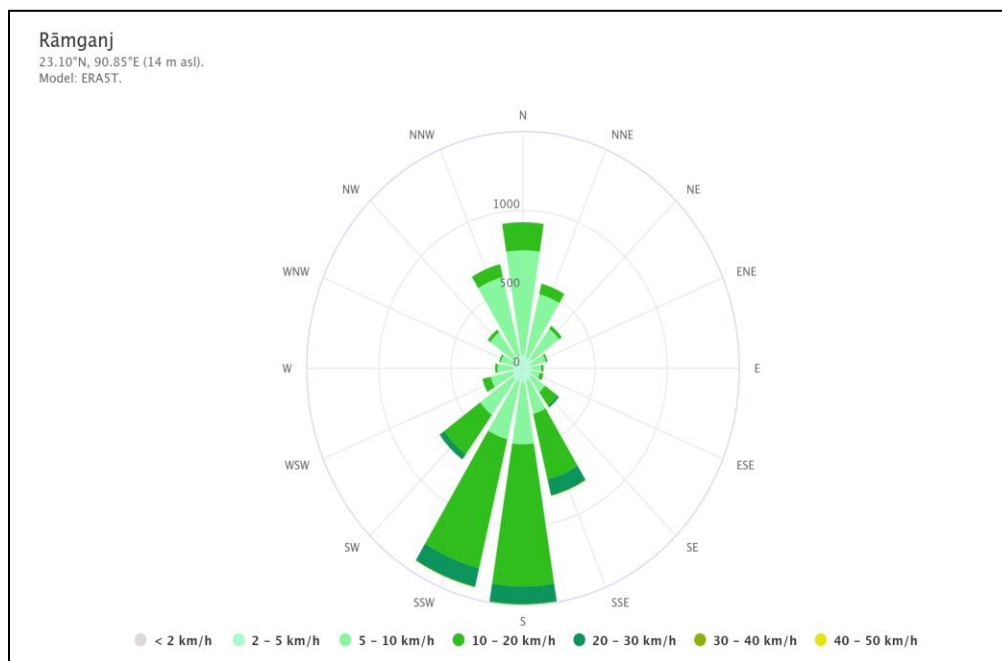
Figure IV-4: Wind Rose*
