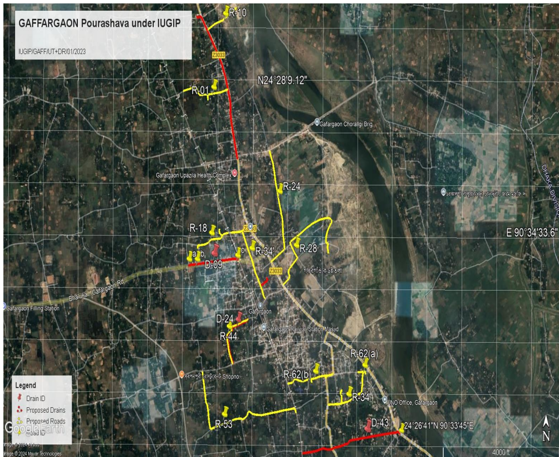
Figure III-5: Location of Roads and Drains at Gaffargaon Pourashava
