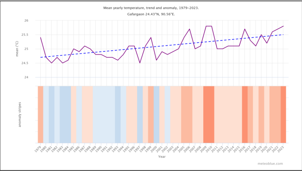
Figure IV-1: Yearly Temperature Change*
