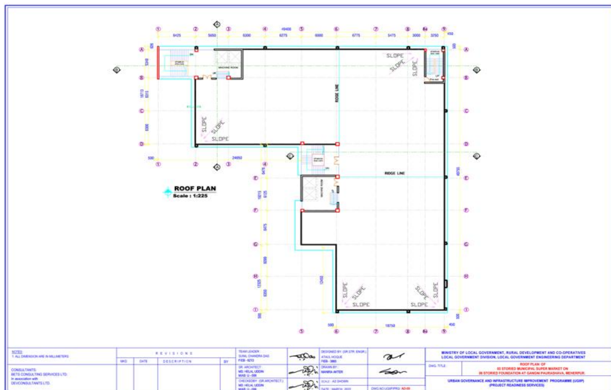
Figure 12: Roof Top Plan of Proposed Municipal Super Market
