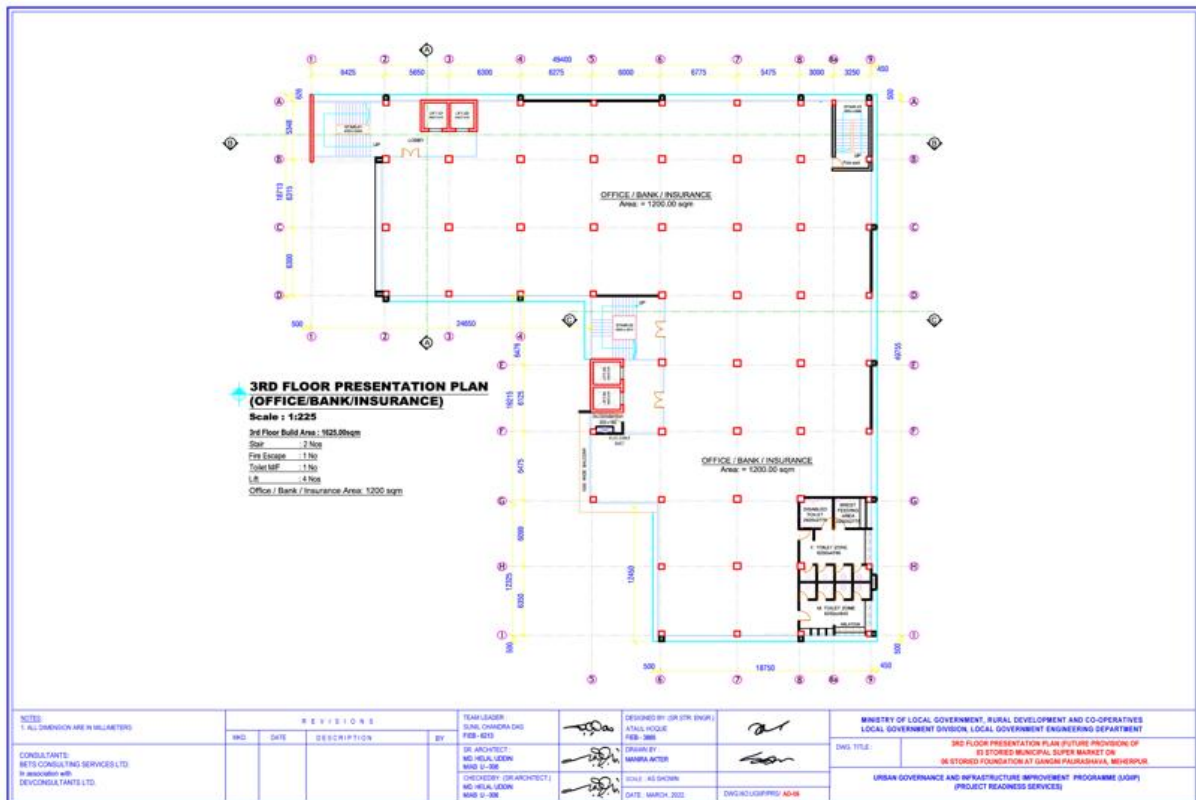
Figure 9: 3 rd Floor Plan of Proposed Municipal Super Market
