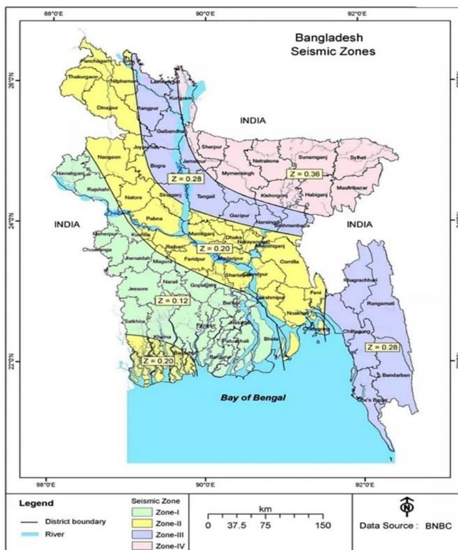
Figure 15: Earthquake Zone in Bangladesh
