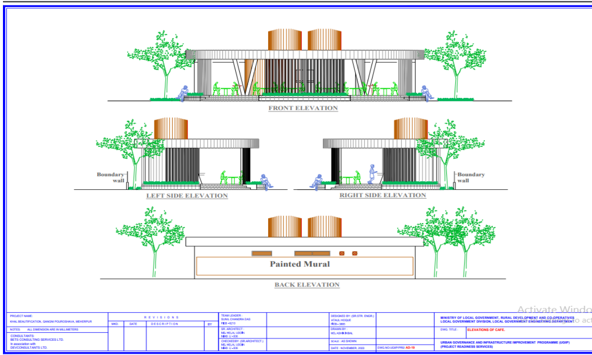
Figure 9: Elevation of Proposed Municipal Lake Beautification
