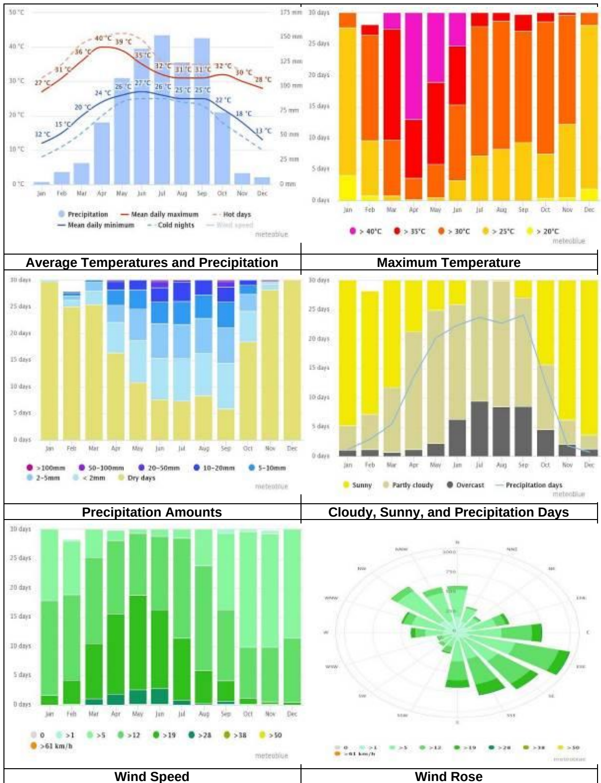
Figure 15: Historical Climatic Record at Meherpur Region
