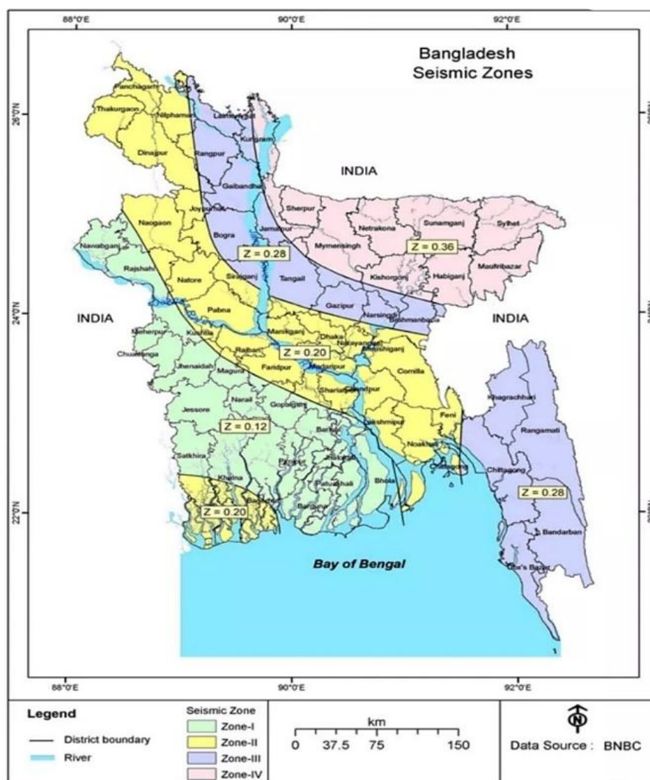
Figure 16: Earthquake Zone in Bangladesh
