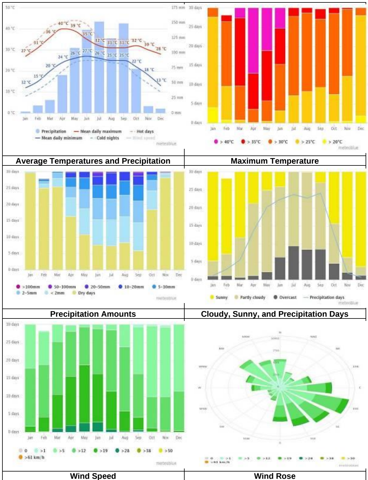
Figure 7: Historical Climatic Record at Meherpur Region
