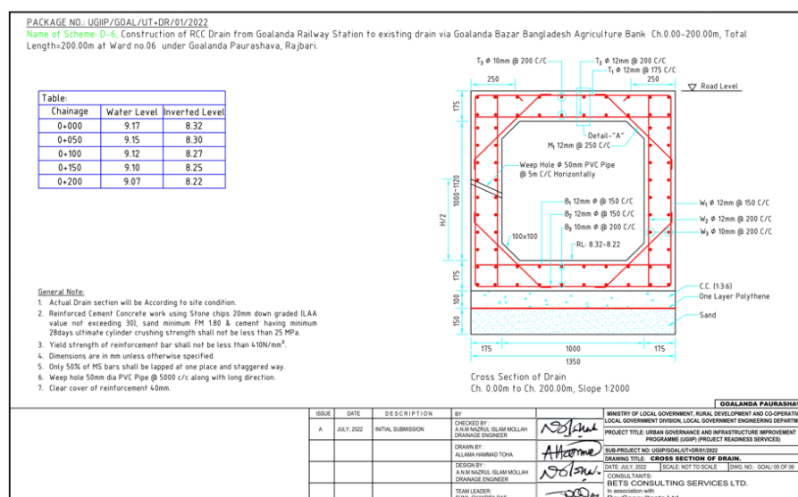
Figure III-6: Cross Section of Drain in Goaland Pourashava
