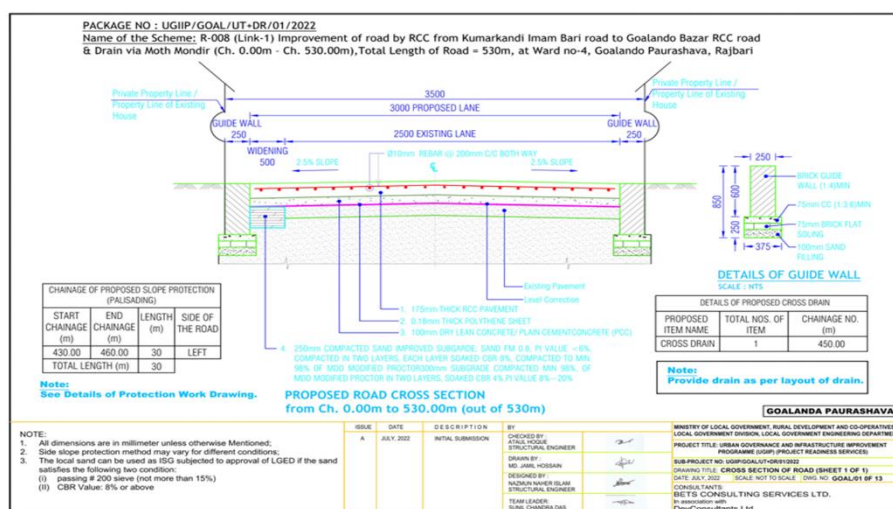
Figure III-5: Cross Section of Road in Goaland Pourashava
