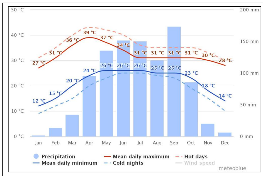
Figure IV-1: Average Temperature & Precipitation
