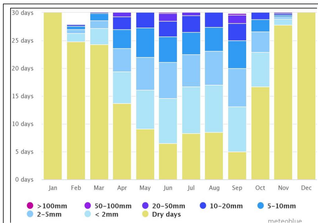
Figure IV-2: Precipitation Amount*
