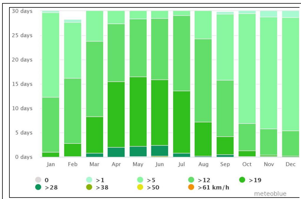
Figure IV-3: Wind Speed*
