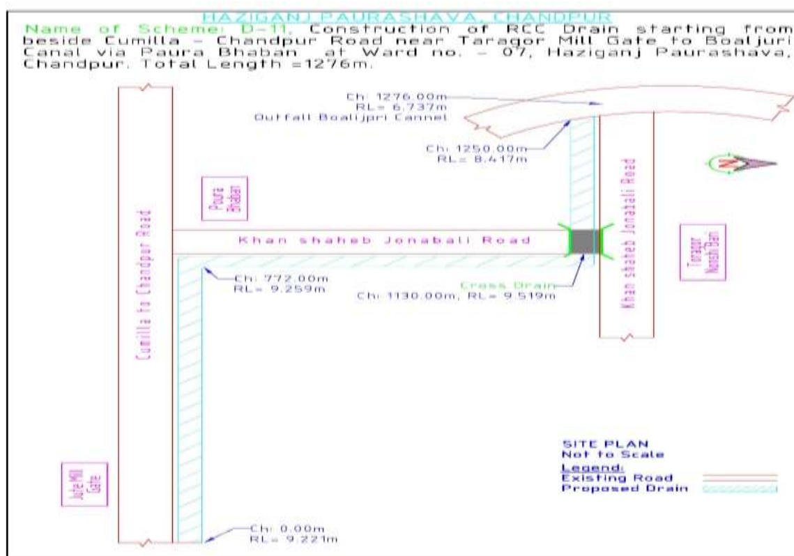
Figure 3: Layout plan of Drain at Haziganj Pourashava
