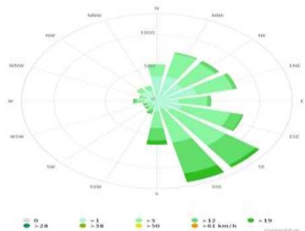
Wind Rose
