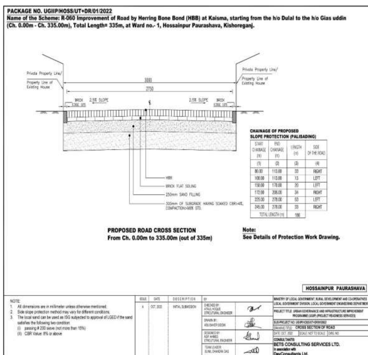
Figure 4: Cross-Section of Road in Hossainpur Paurashava
