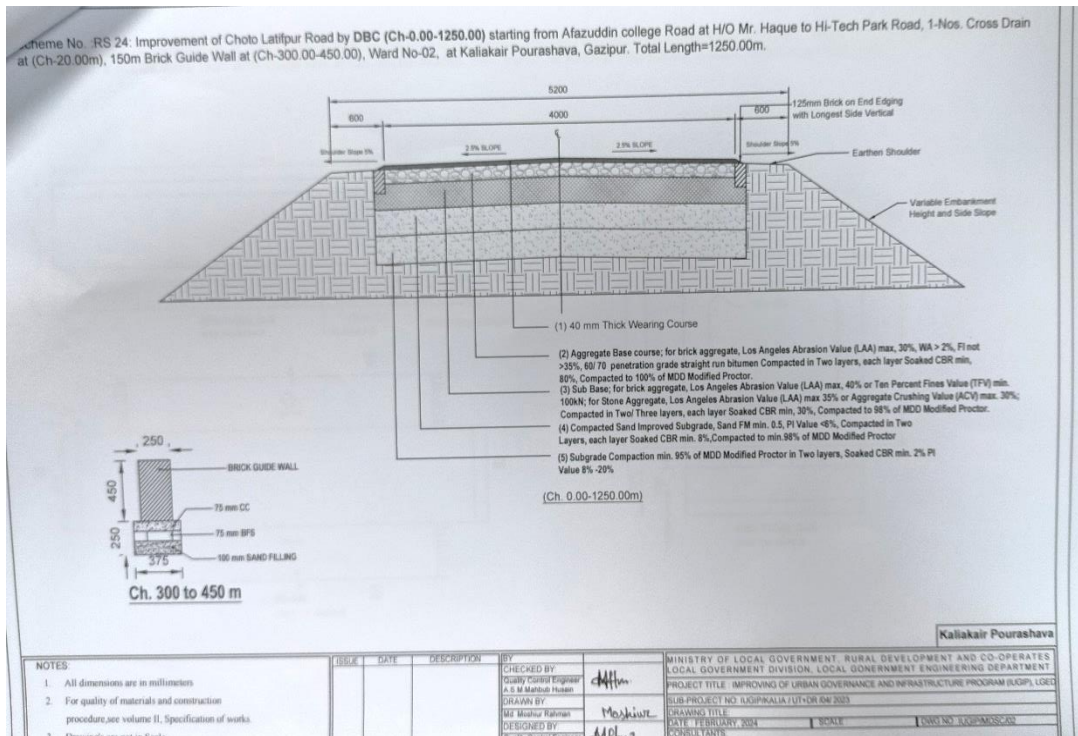
Figure 4: Cross-Section of Road in Kaliakair Pourashava
