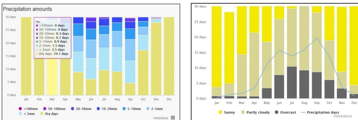
Precipitation Amounts
