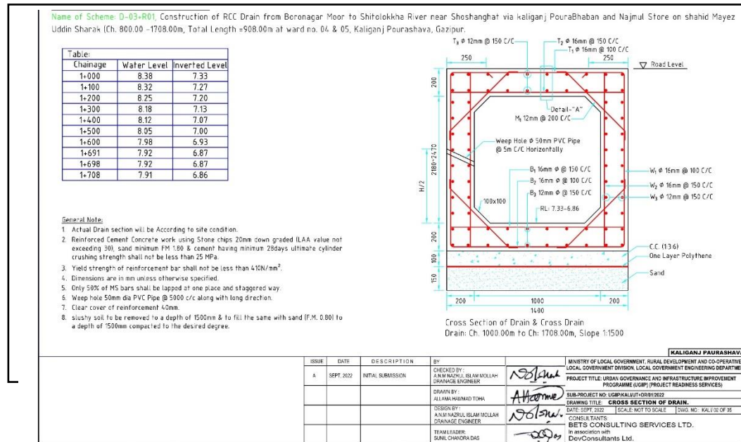
Figure III-5: Cross Section of Drain in Kaliganj Pourashava
