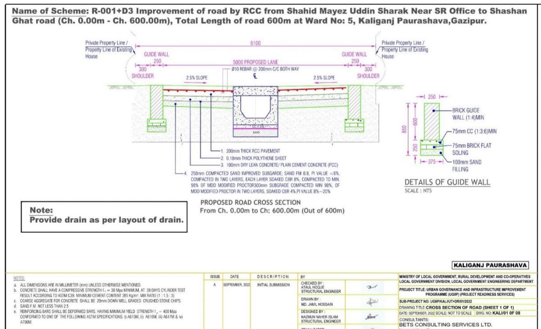
Figure III-4: Cross Section of Road in Kaliganj Pourashava
