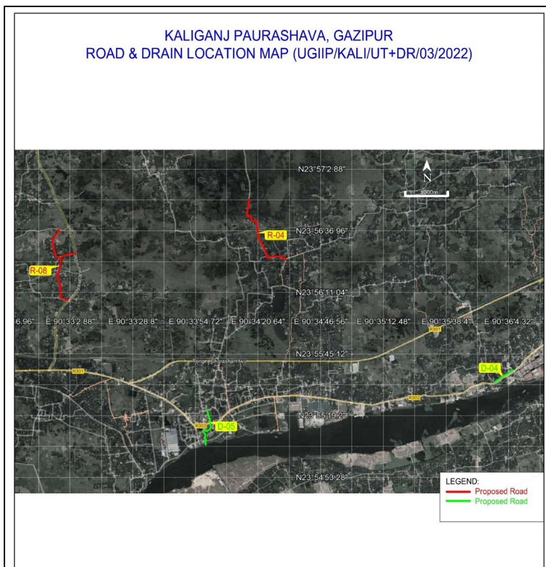
Figure III-6: Location of Roads, Drains at Kaliganj Pourashava
