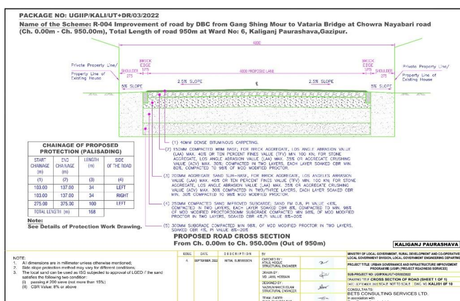
Figure III-4: Cross Section of Road in Kaliganj Pourashava
