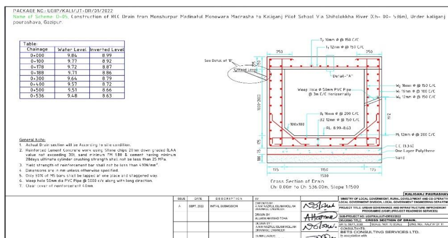
Figure III-5: Cross Section of Drain in Kaliganj Pourashava
