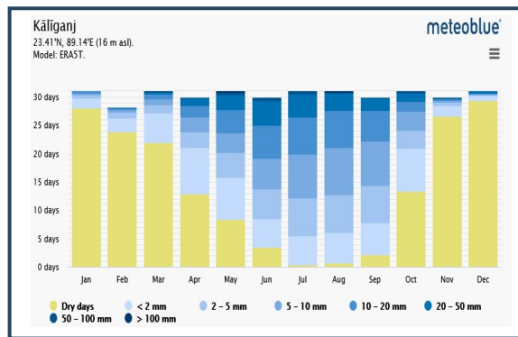
Precipitation Amounts
