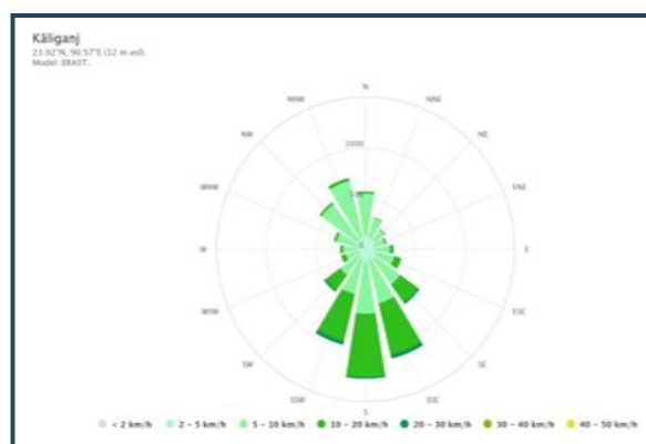
Wind Rose
