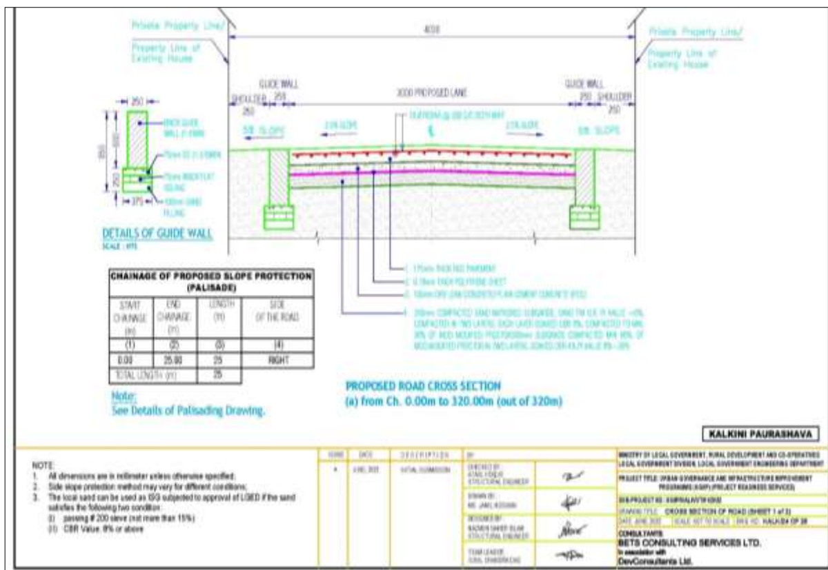
Figure 6: Cross-Section of Road (001) in Pourashava
