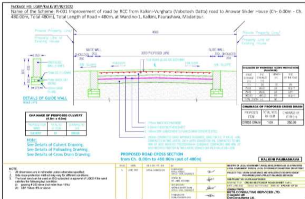
Figure 6: Cross-Section of Road (001) in Pourashava
