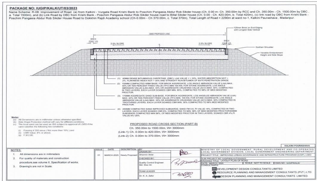
Figure 4: Cross-Section of Road in Kalkini Pourashava
