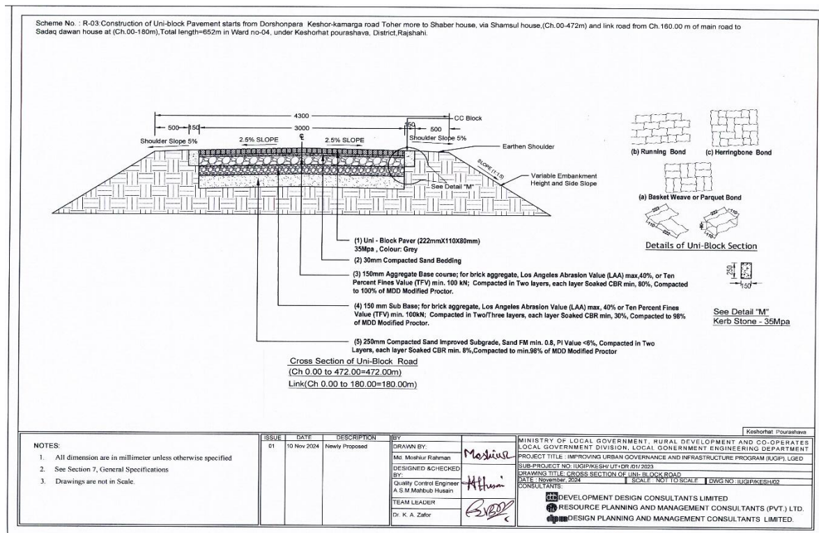
Figure 4: Cross-Section of Road in Pourashava
