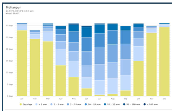
Precipitation Amounts
