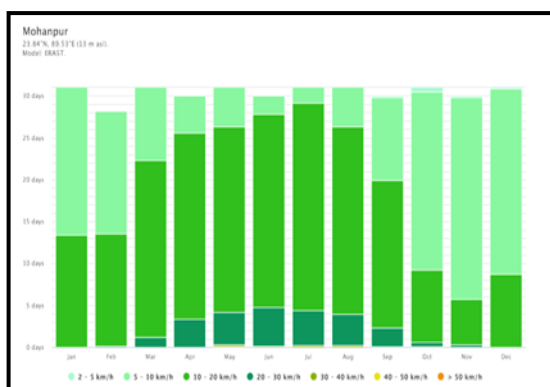
Wind Speed
