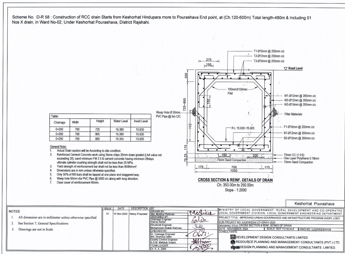
Figure 5: Cross-Section of Drain in Pourashava
