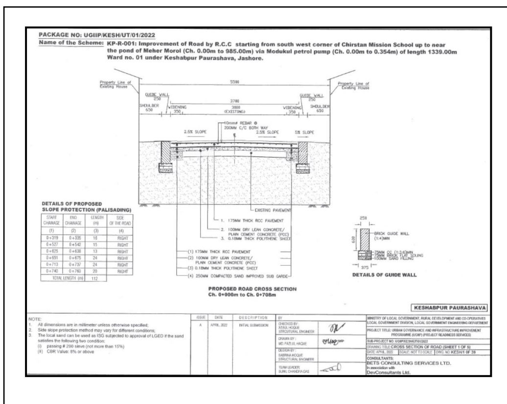
Figure III-3: Cross Section of Road in Keshabpur Pourashava
