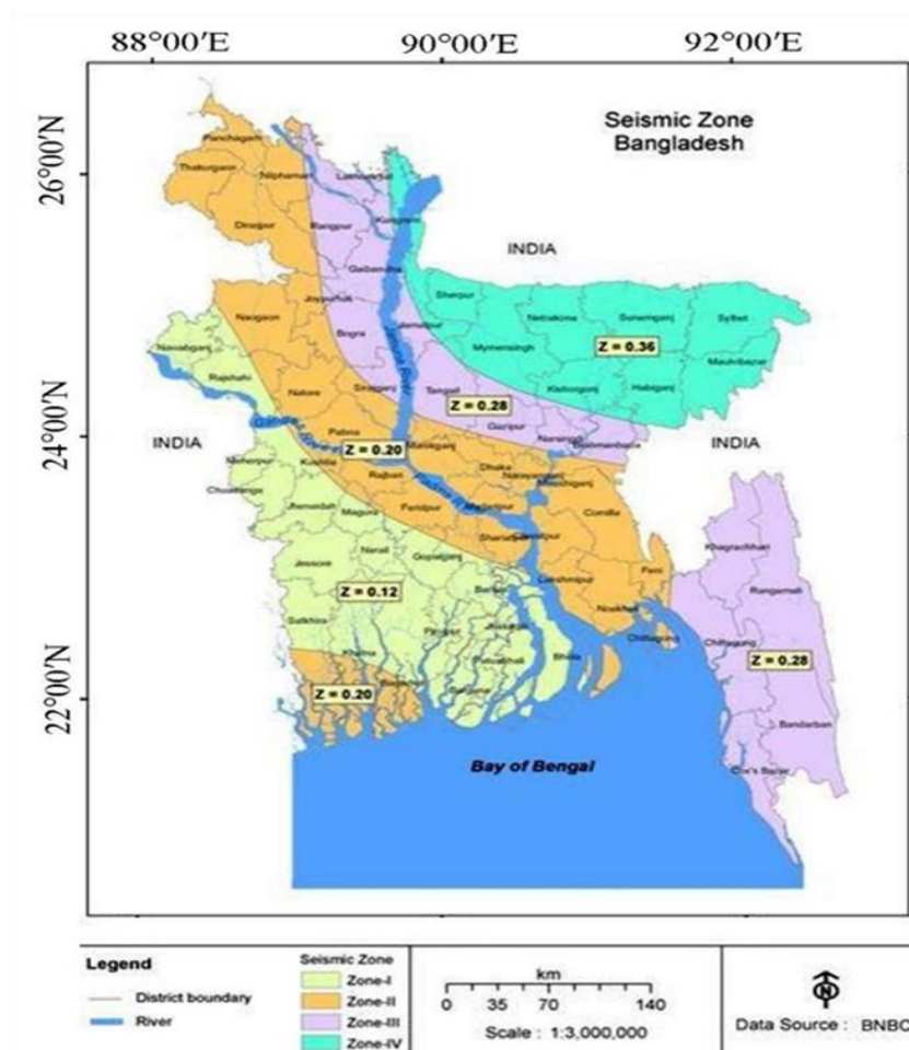
Figure IV-5: Seismic Zones of Bangladesh (4 Zones) [Source: BNBC]
