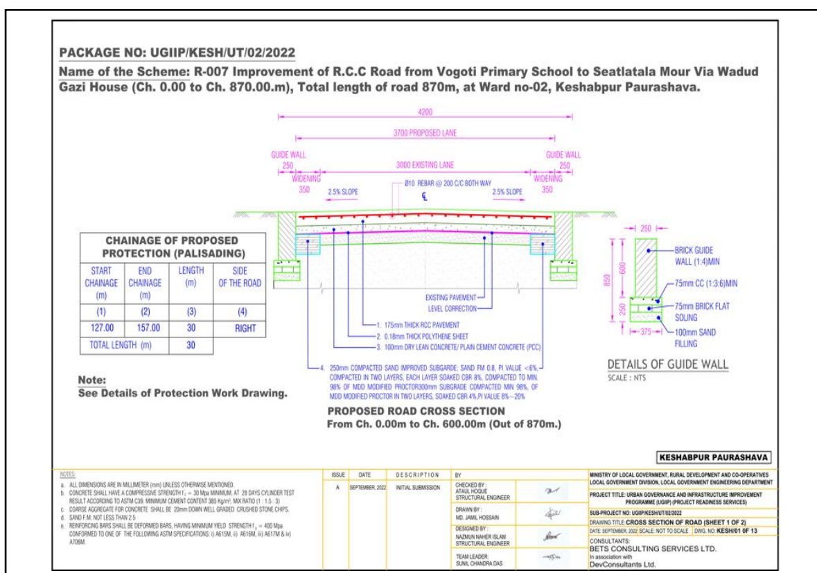
Figure III-3: Cross Section of Road in Keshabpur Pourashava
