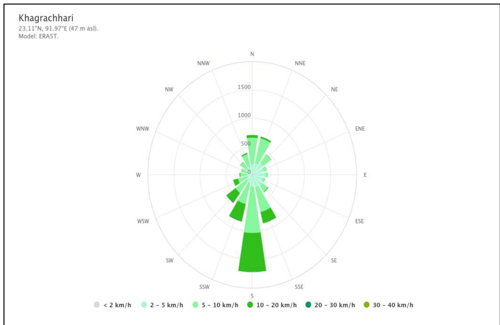
Figure IV-4: Wind Rose*
