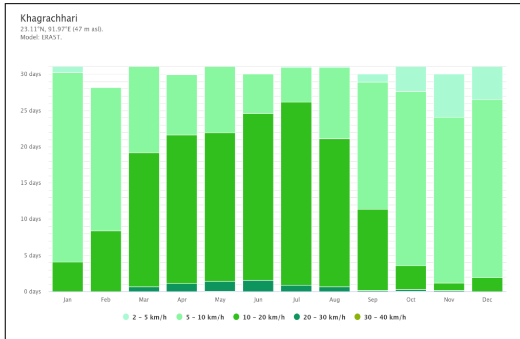
Figure IV-3: Wind Speed*
