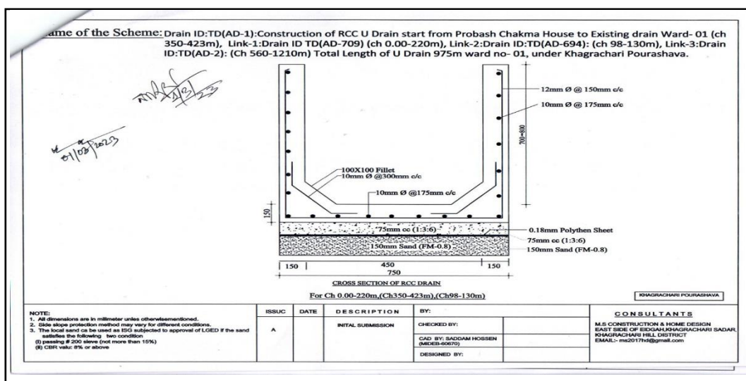
Figure III-6: Cross Section of Drain in Khagrachari Pourashava
