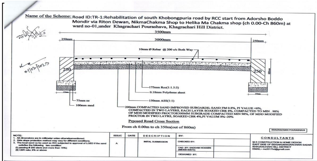
Figure III-5: Cross Section of Road in Khagrachari Pourashava
