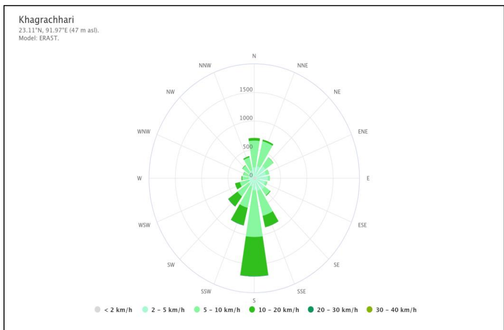
Figure IV-4: Wind Rose*
