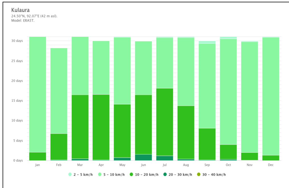
Figure IV-III: Wind Speed*
