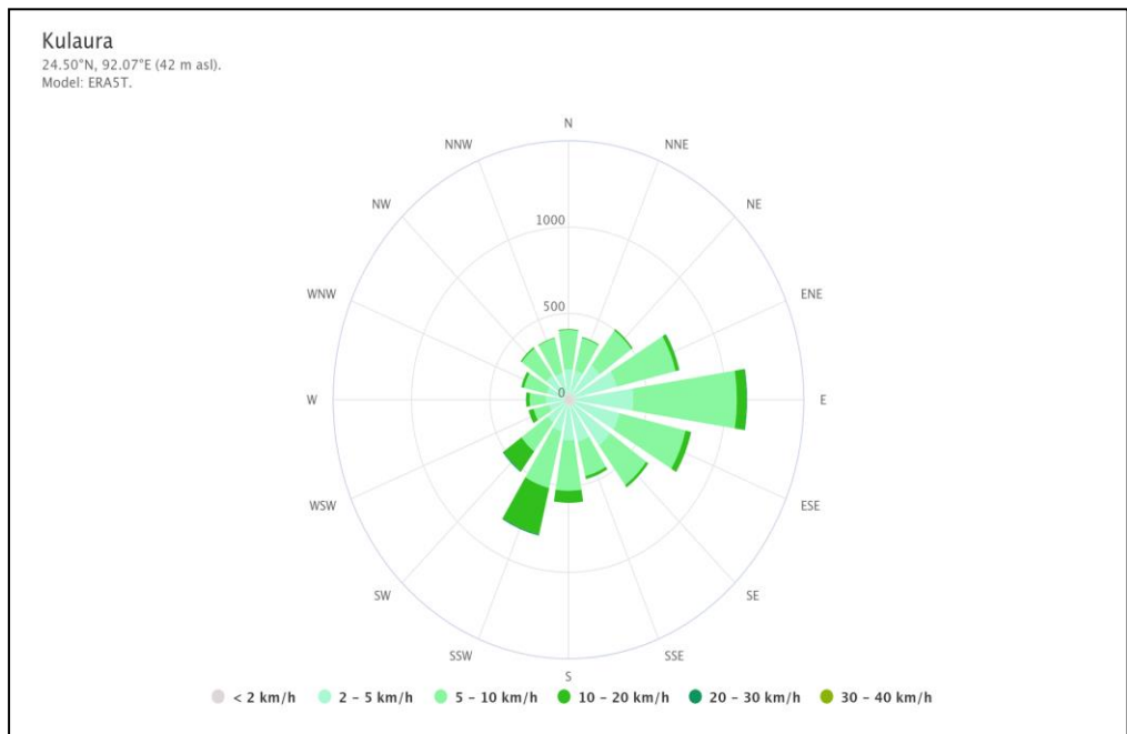
Figure IV-IV: Wind Rose*
