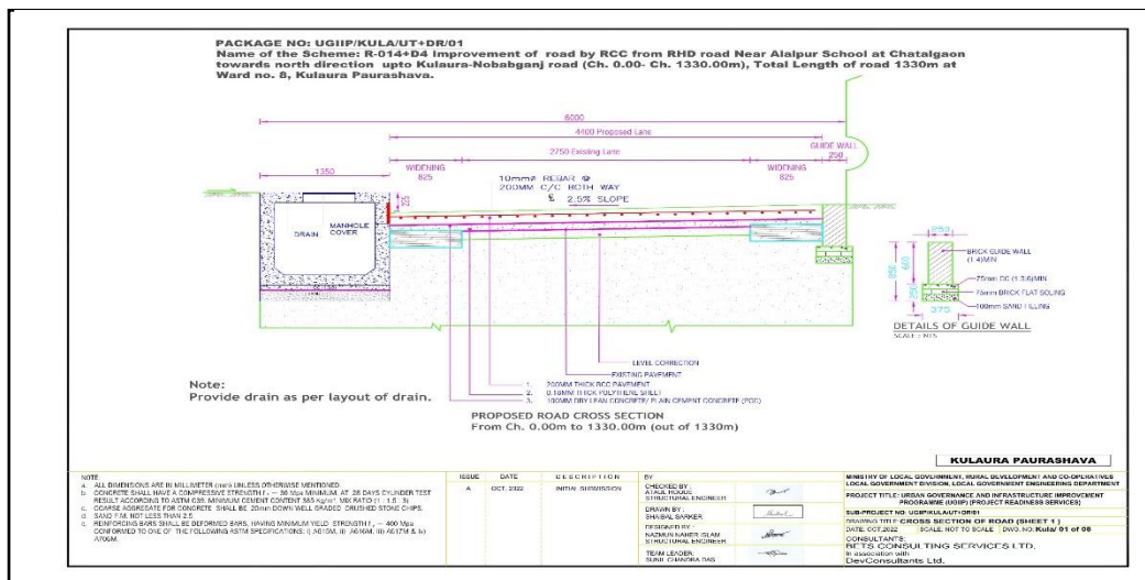
Figure III-V: Cross Section of Road in Kulaura Pourashava
