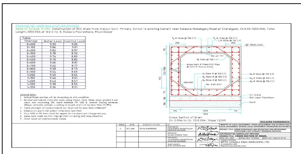
Figure III-VI: Cross Section of Drain in Kulaura Pourashava
