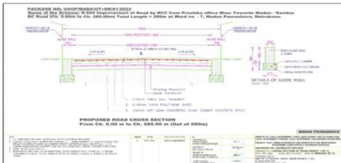
Figure 6: Cross-Section of Road in Pourashava
