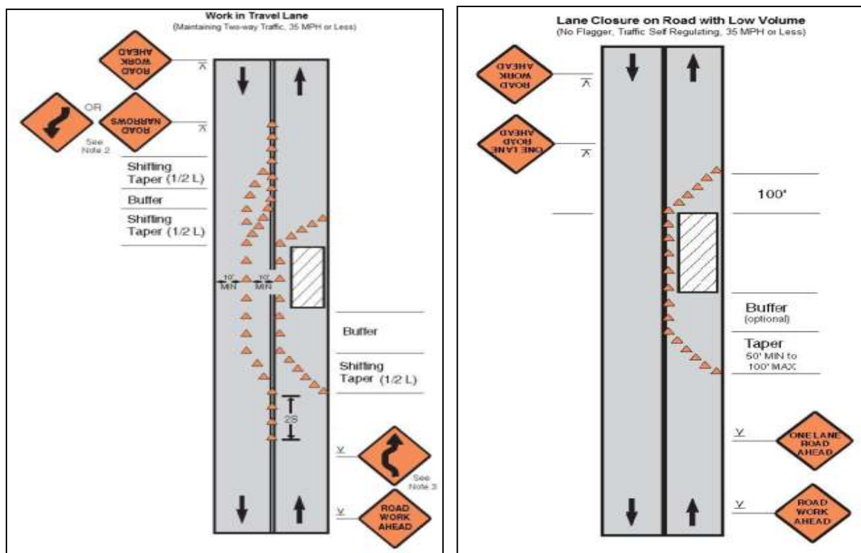
Figure A4 & A5: Work in Travel lane & Lane closure on road with low volume
