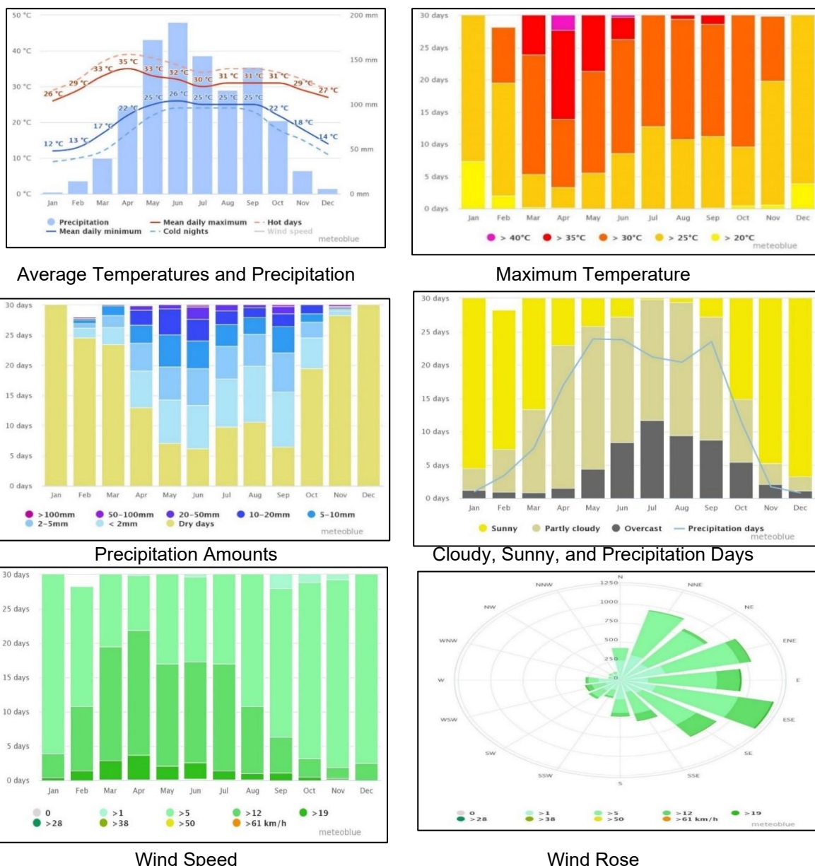
Figure 5: Historical Climatic Record at Madan Region
