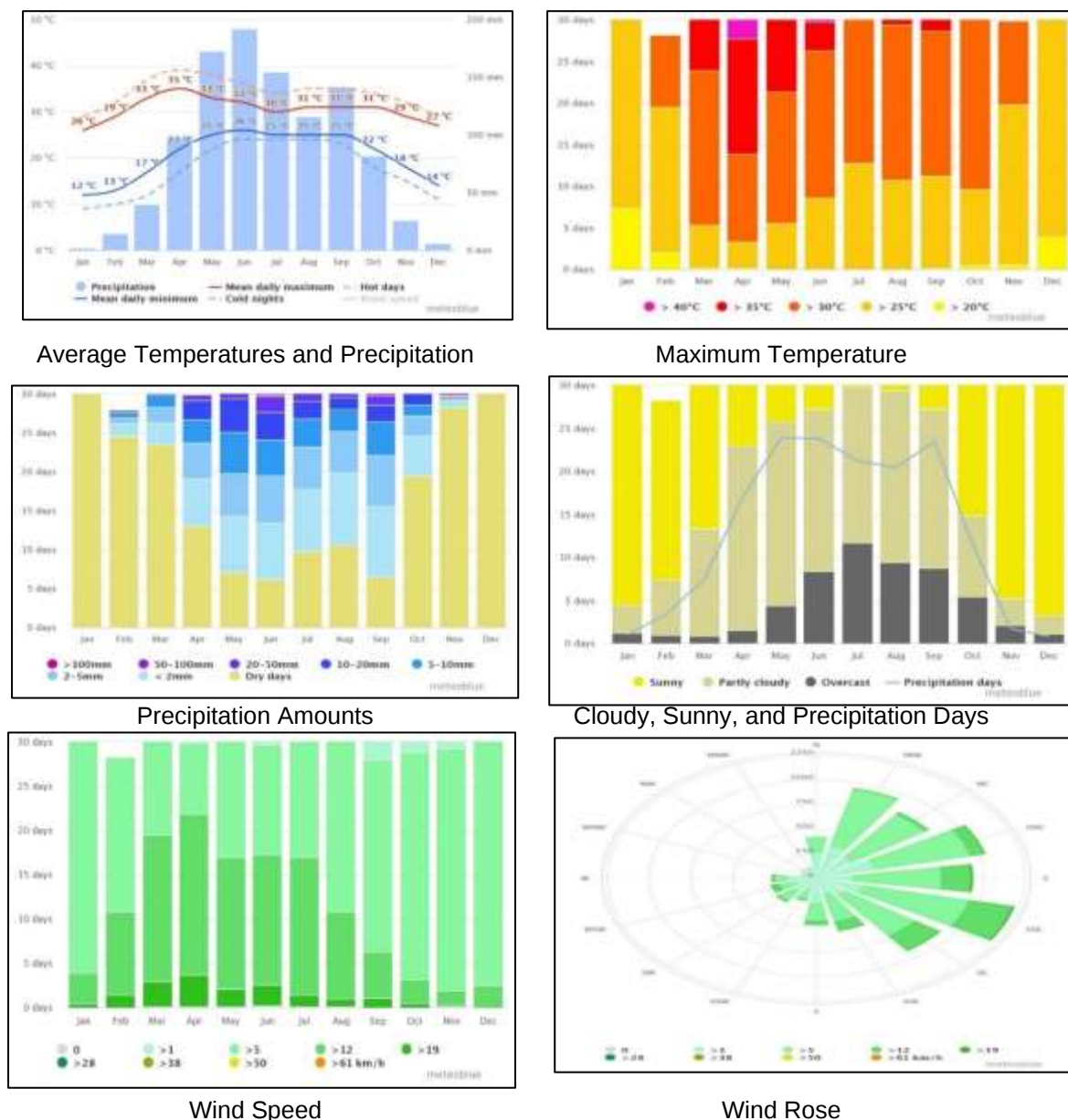
Figure 7: Historical Climatic Record at Madan Region
