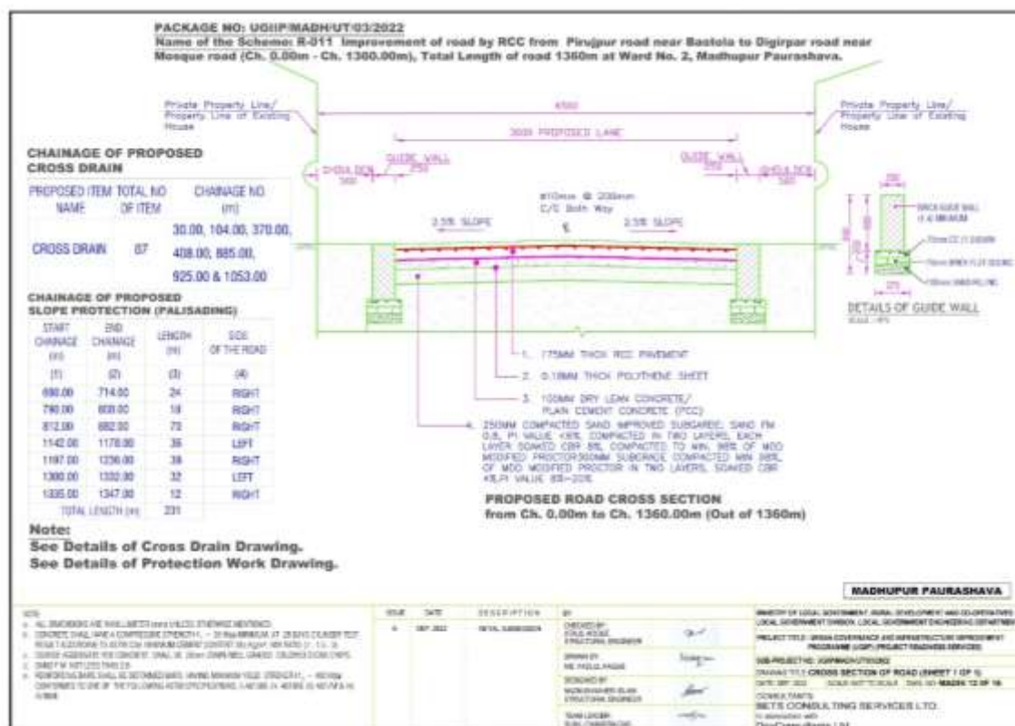
Figure 6: Cross-Section of Road in Pourashava
