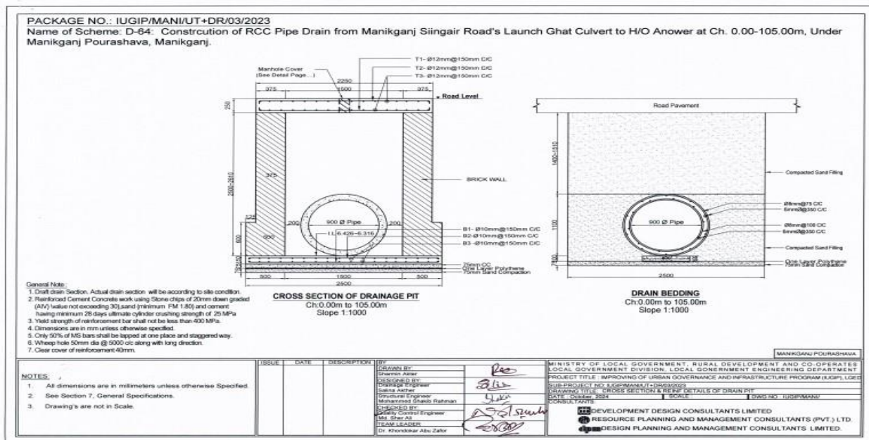
Figure 4: Cross-Section of Drain in Pourashava
