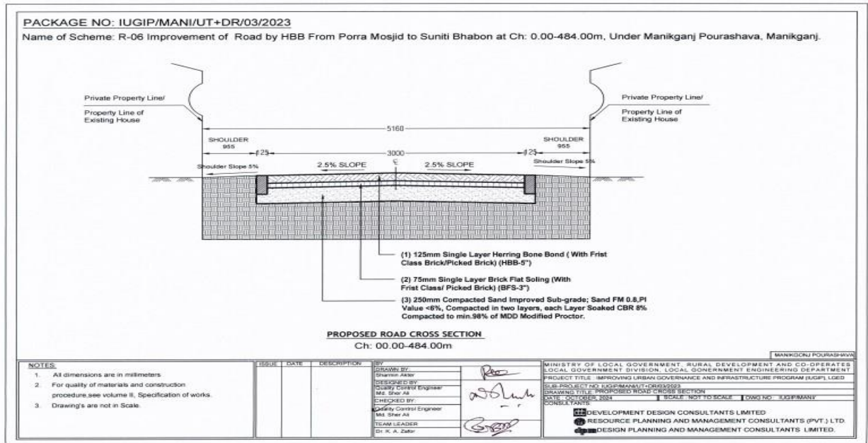
Figure 3: Cross-Section of Road in Pourashava
