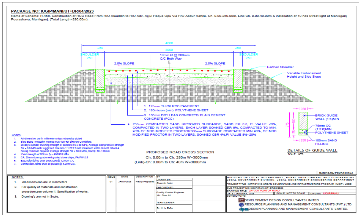
Figure 3: Cross-Section of Road in Pourashava
