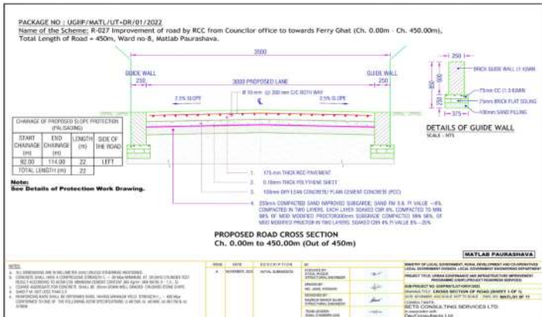
Figure 3: Cross section of Road at Matlab Pourashava
