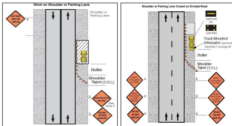
Figure A2 & A3: Work on shoulder or parking lane and shoulder or parking lane closed on divided road
