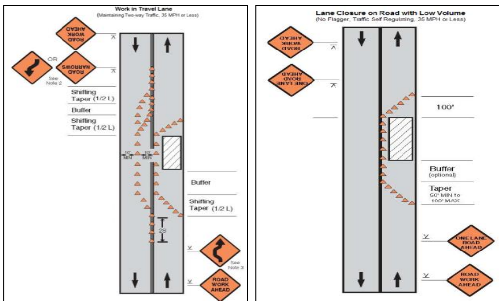
Figure A4 & A5: Work in Travel lane & Lane closure on road with low volume
