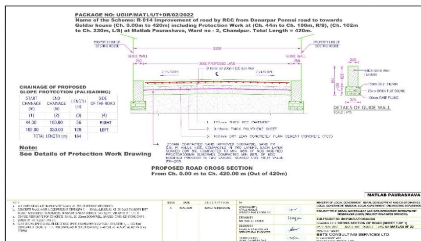
Figure 3: Cross section of Road at Matlab Pourashava
