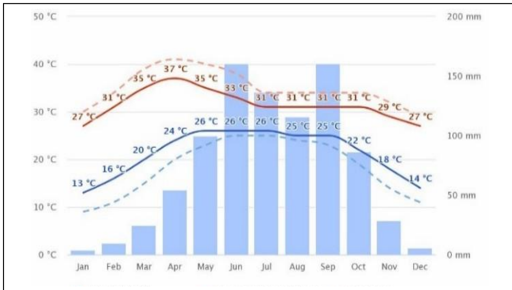
Figure IV-1: Average Temperatures and Precipitation*
