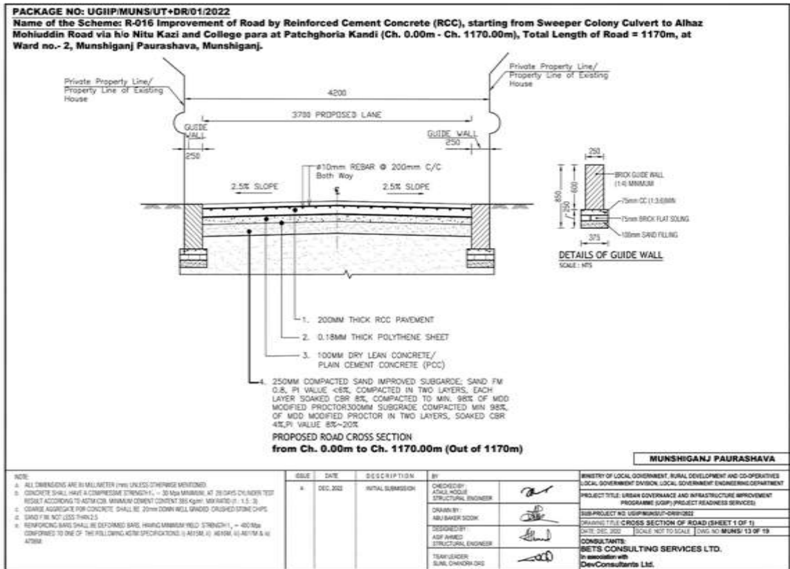
Figure 3: Cross section of Road at Munshiganj Pourashava
