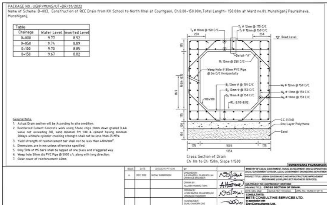
Figure 4: Cross-Section of Drain in Mnshiganj Pourashava
