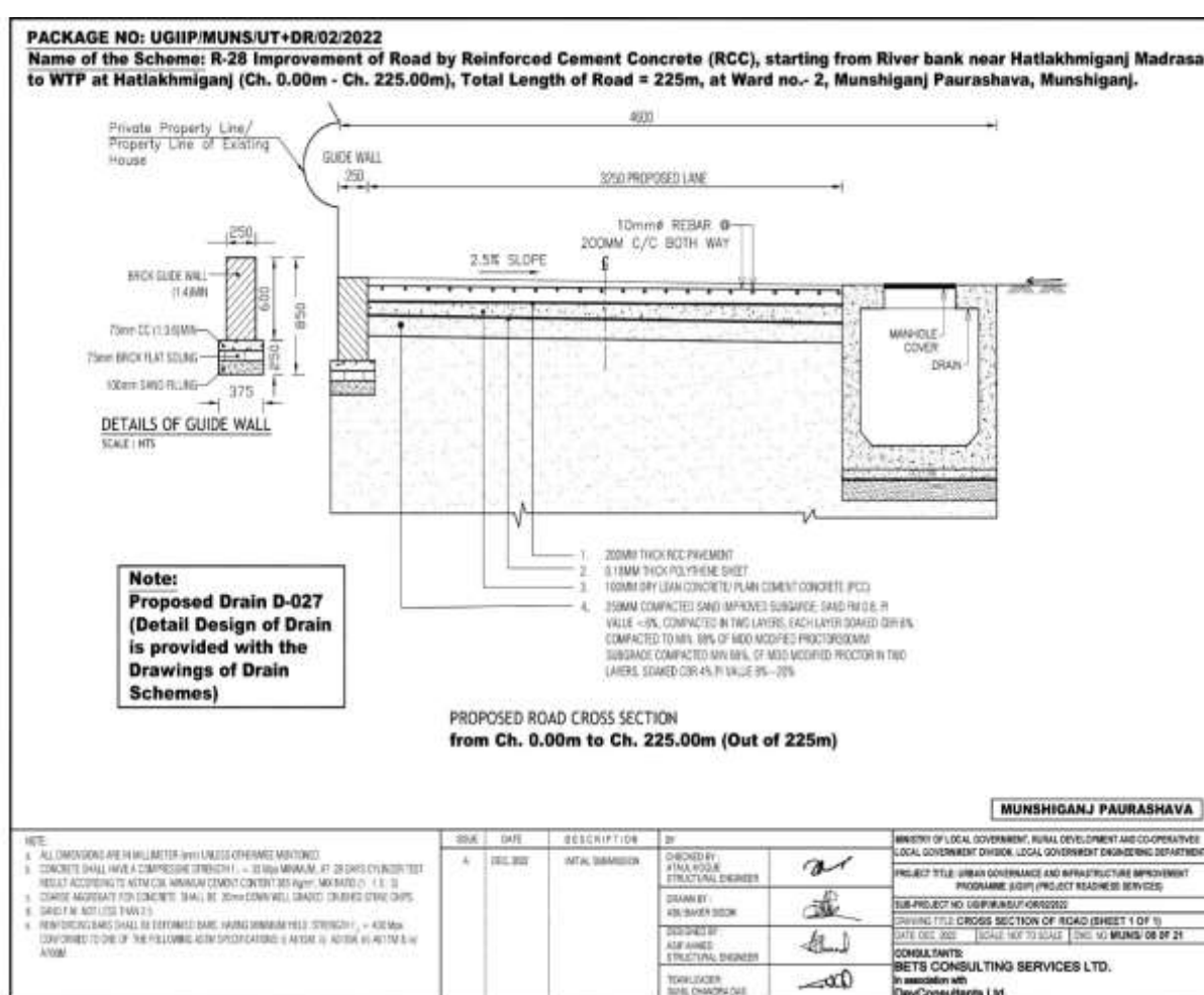
Figure 3: Cross section of Road at Munshiganj Pourashava
