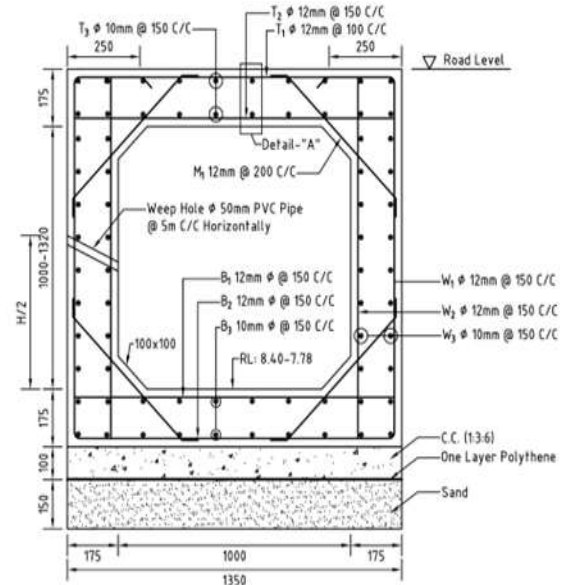
Cross Section of Drain, Ch: 619m to Ch: 0m, Slope 1:1000 Cross Drain, Ch: 619m to Ch: 613m (Size 1000mmX1000mm), Slope 1:1000
