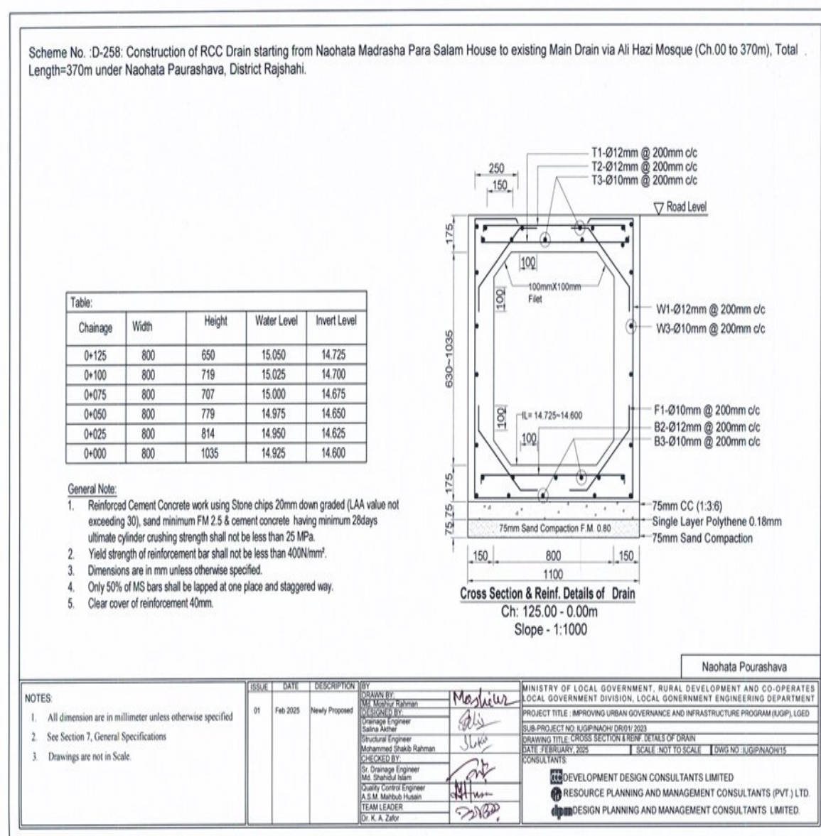
Figure 5: Cross-Section of Drain in Pourashava
