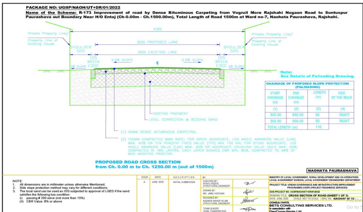
Figure 3: Cross-Section of Road Naohata Paurashava
