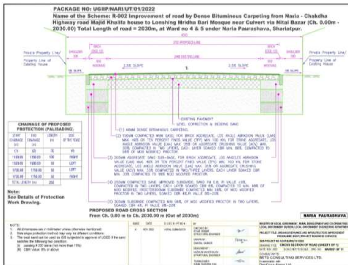
Figure 5: Cross-Section of Road in Pourashava
