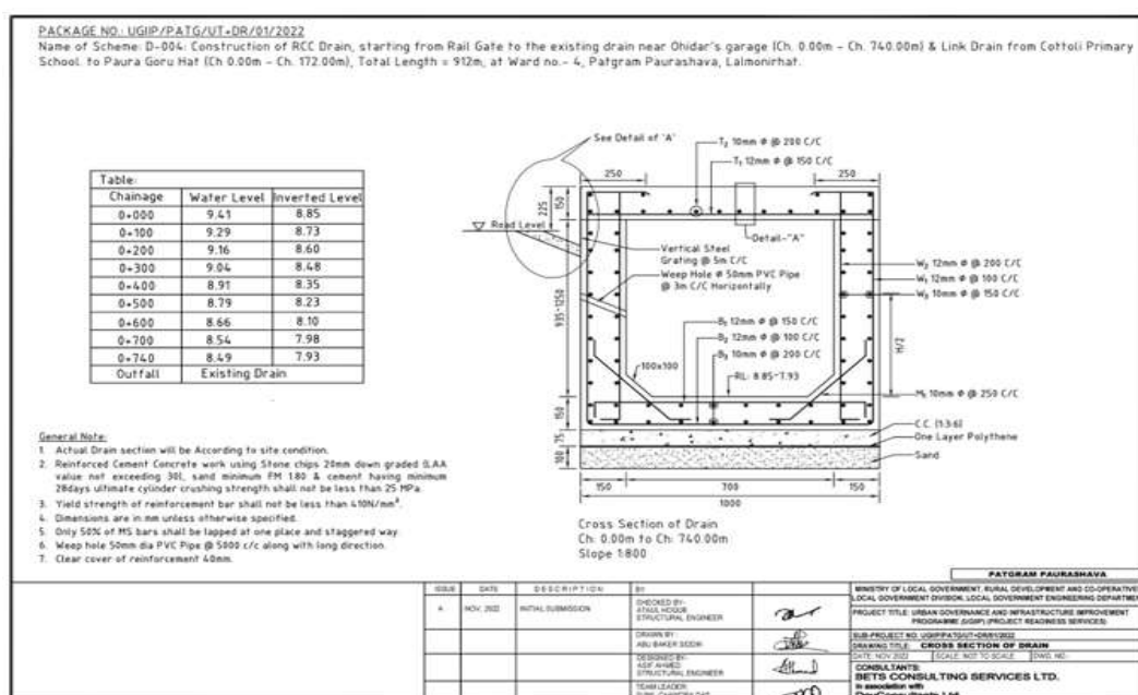
Figure 6: Cross-Section of Drain in Pourashava
