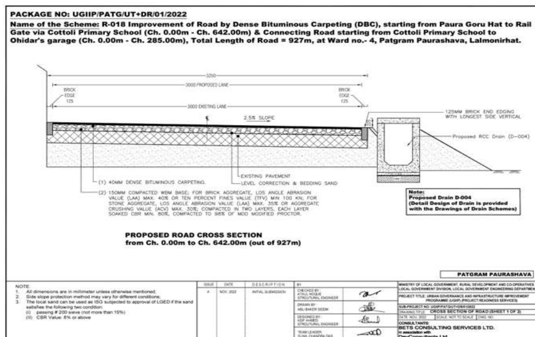
Figure 5: Cross-Section of Road in Pourashava
