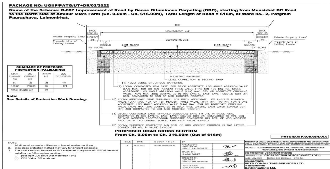
Figure 5: Cross-Section of Road in Pourashava
